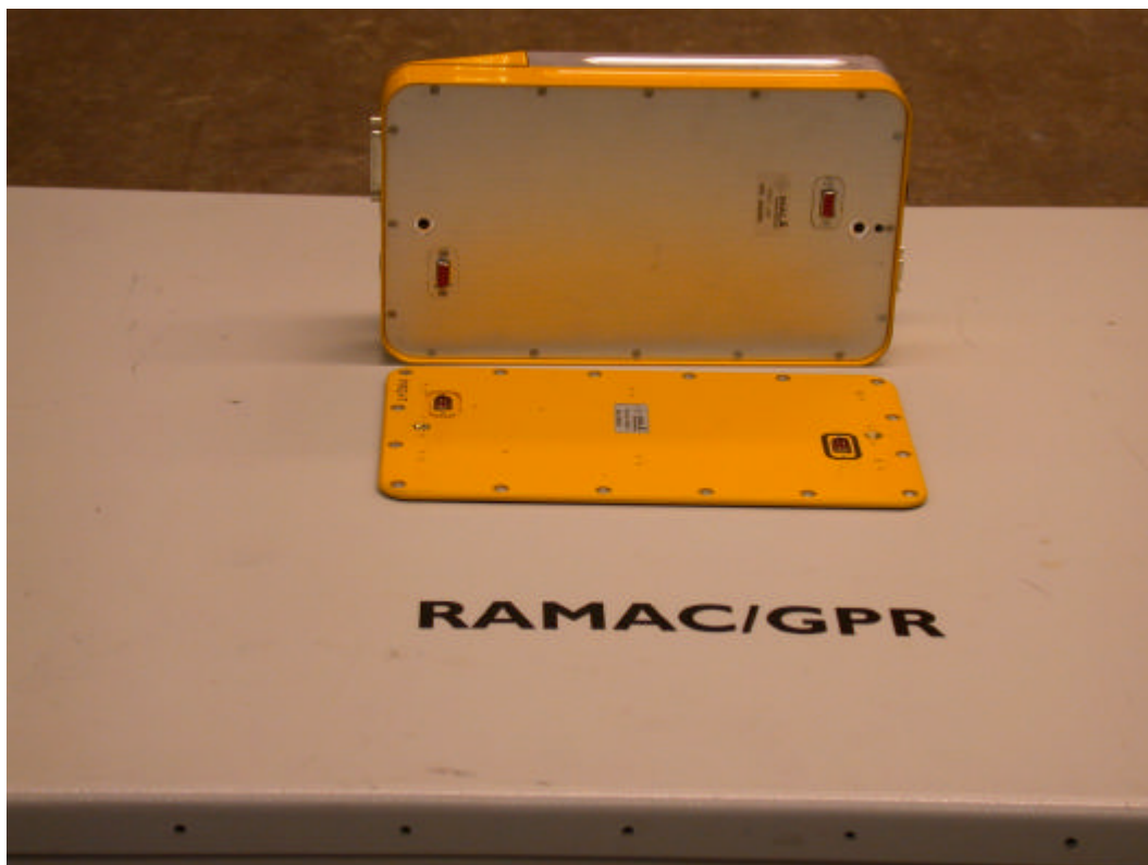
Figure 3. Overview of antenna connectors located on the bottom side of the X3M/EasyLocator and topside of antennas.
