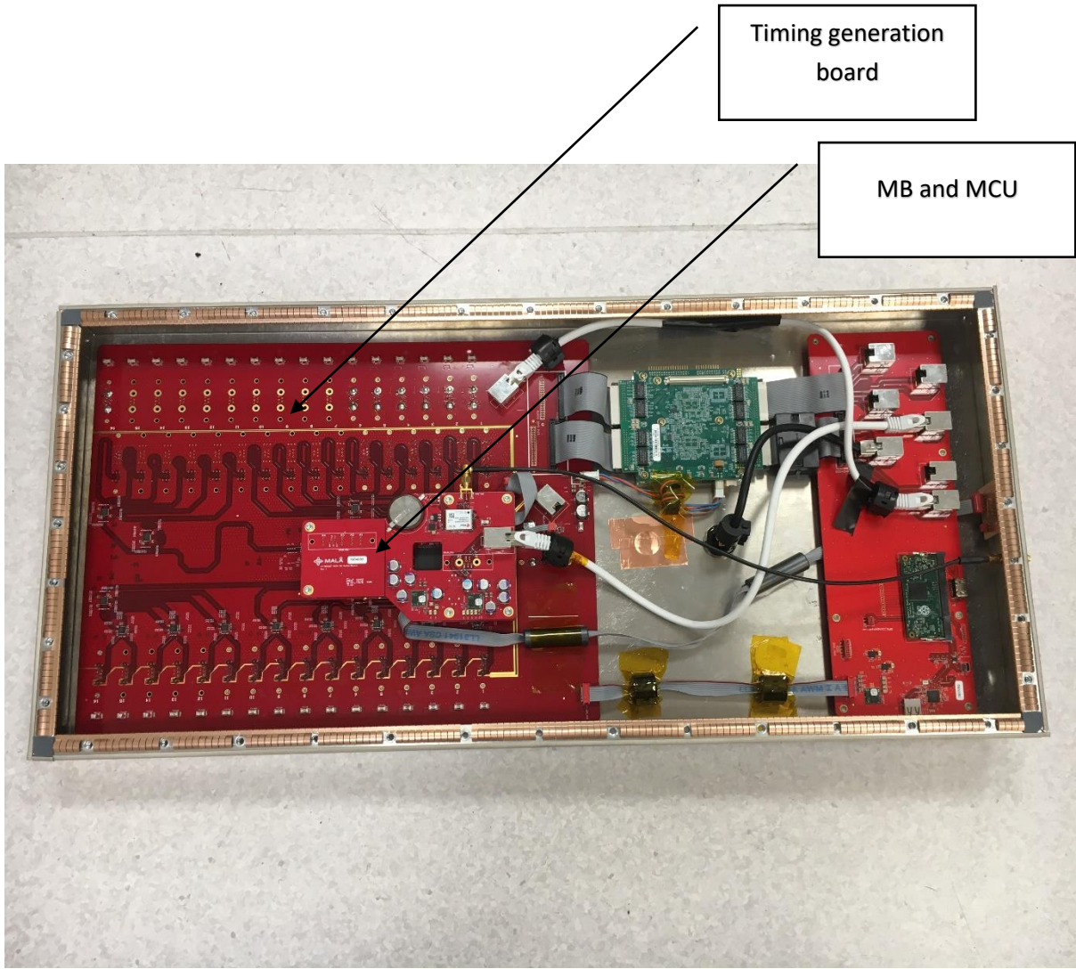
Photo 3: Lid removed from Blockmaster
