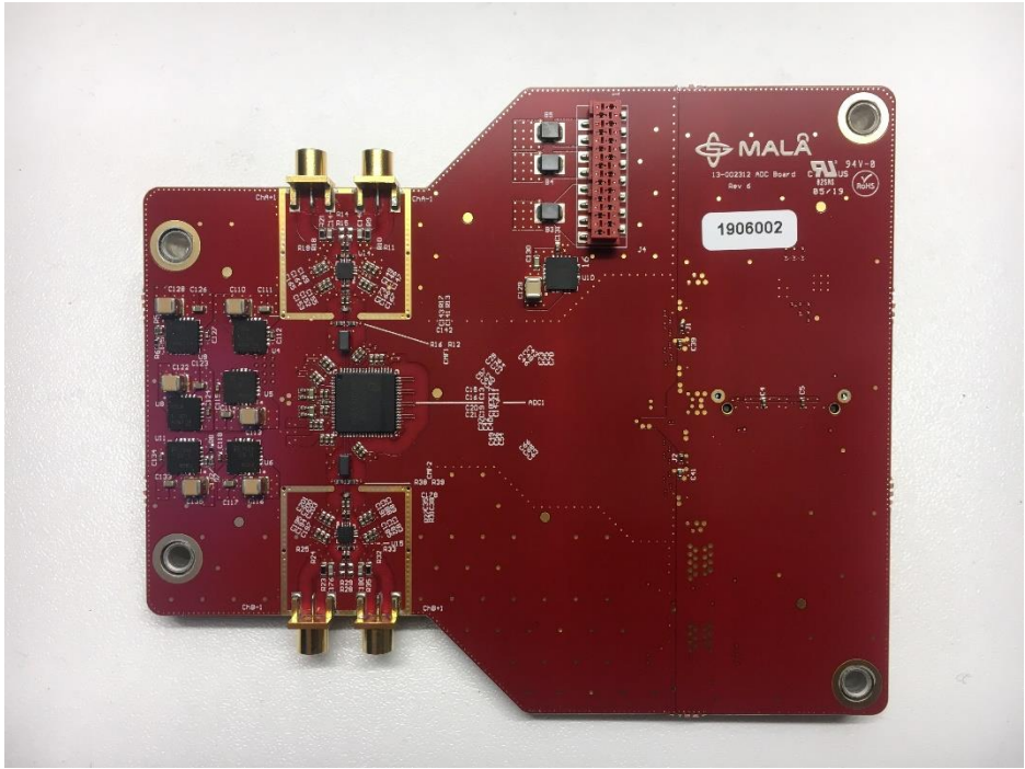
Photo 19: ADC board – front
