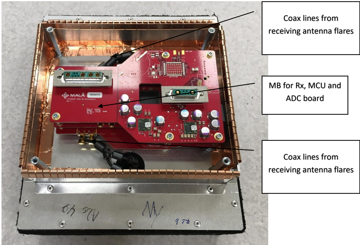
Photo 17: Lid removed
