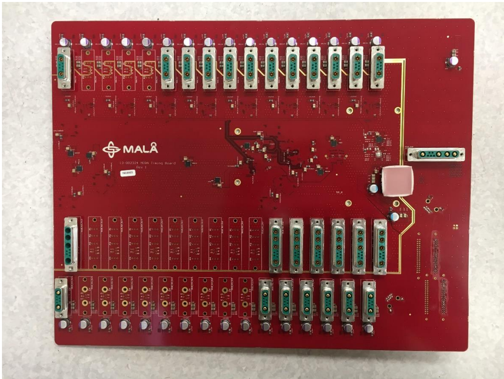
Photo 8: Timing generation board – back
