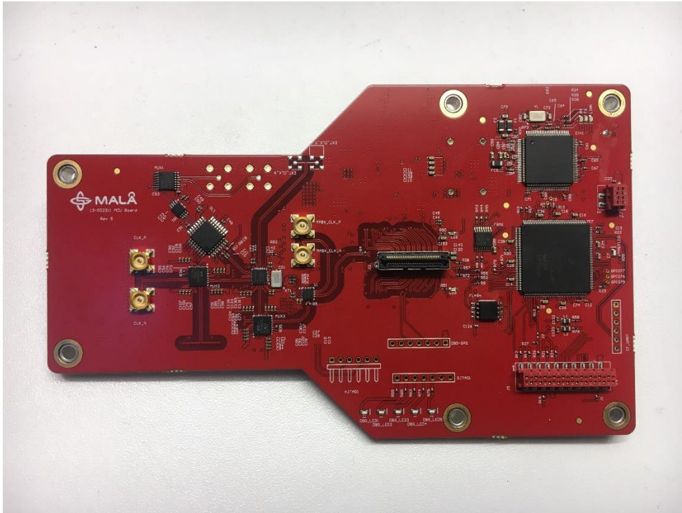
Photo 5: MCU – front
