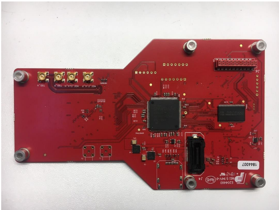
Photo 6: MCU – back
