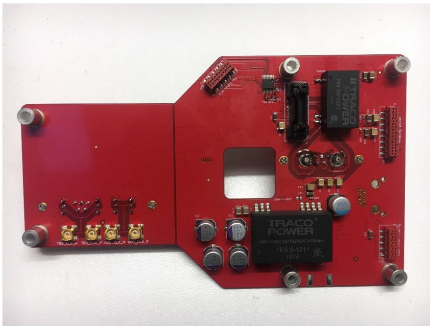
Photo 18: MB RX board – back
