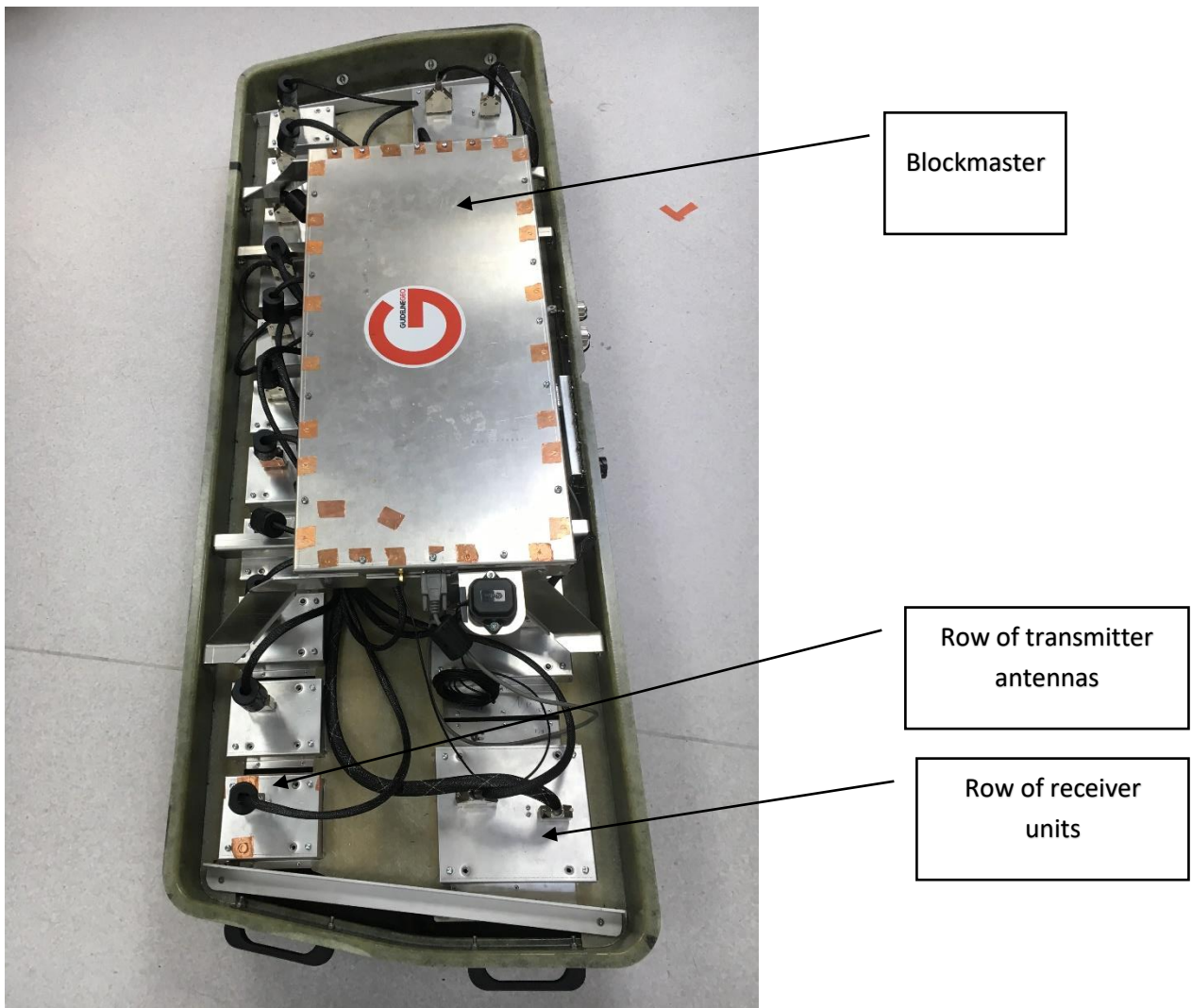
Photo 2: Lid removed, exposing Blockmaster and transmitter and receiver antennas
