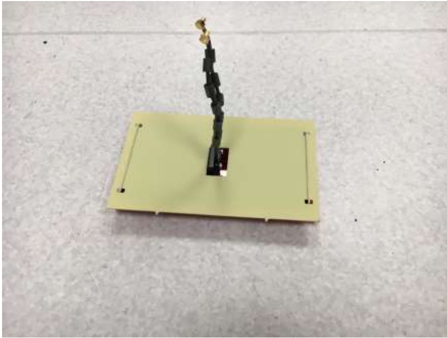
Photo 29: One set of antenna flares removed from antenna
