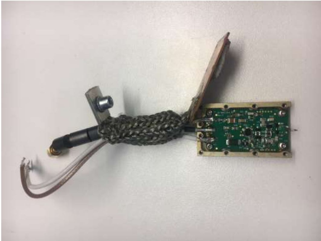
Photo 21: Pulsegenerator - front
