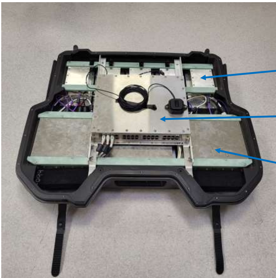
Photo 2: Lid removed, exposing Blockmaster and transmitter and receiver antennas
