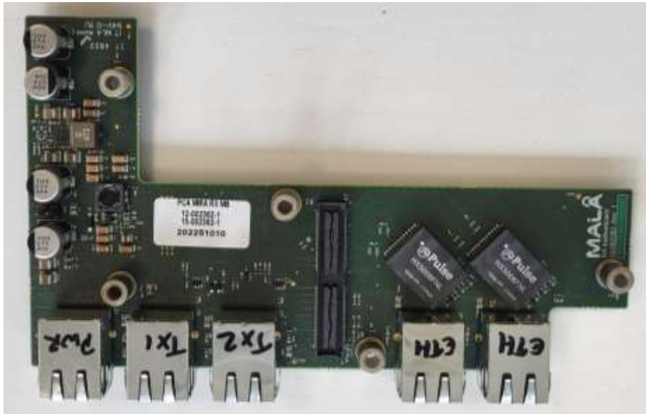
Photo 24: RX motherboard – front
