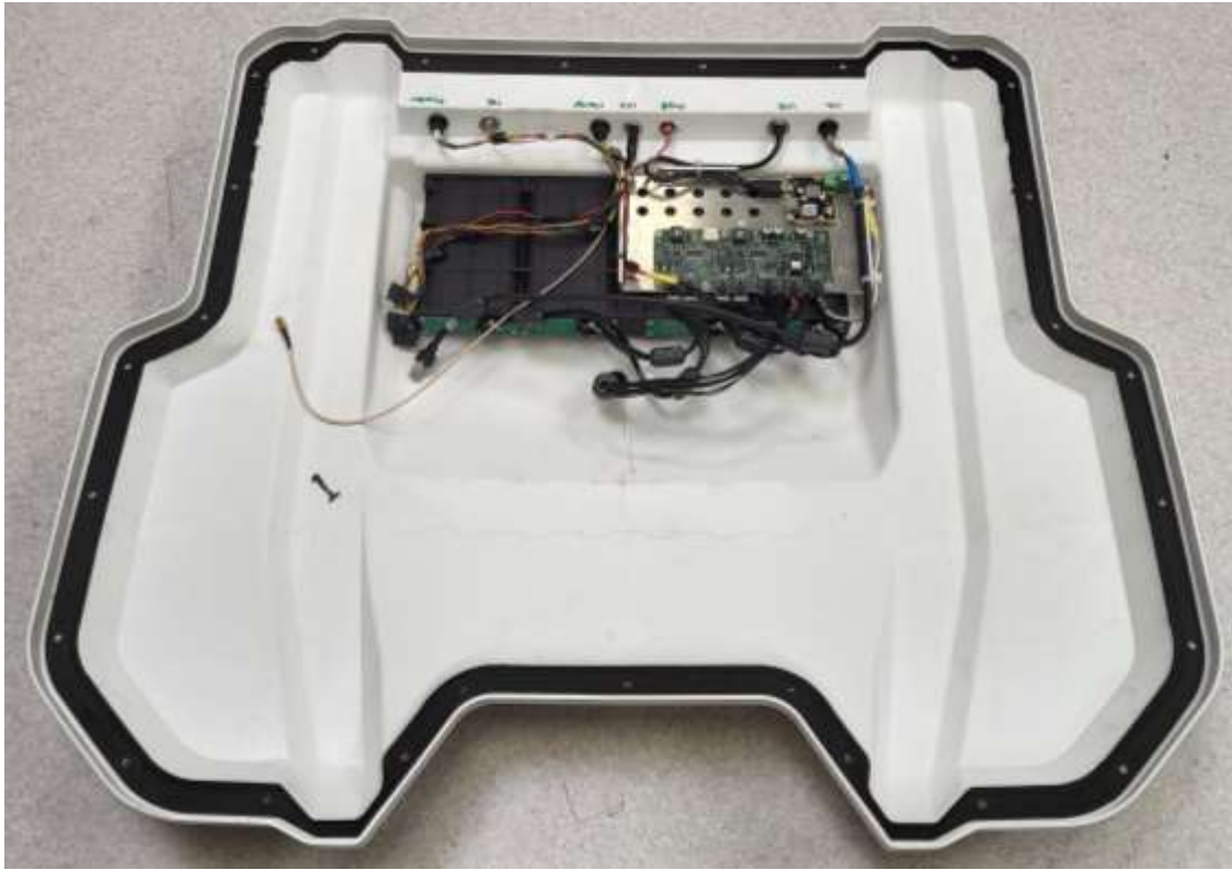
Photo 8: Inside lid, exposing battery compartments, Battery connector boards, Quad battery board and USB-C PD board.
