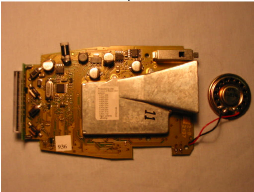
Model: Express 936 FCC ID: QL4G4M2
