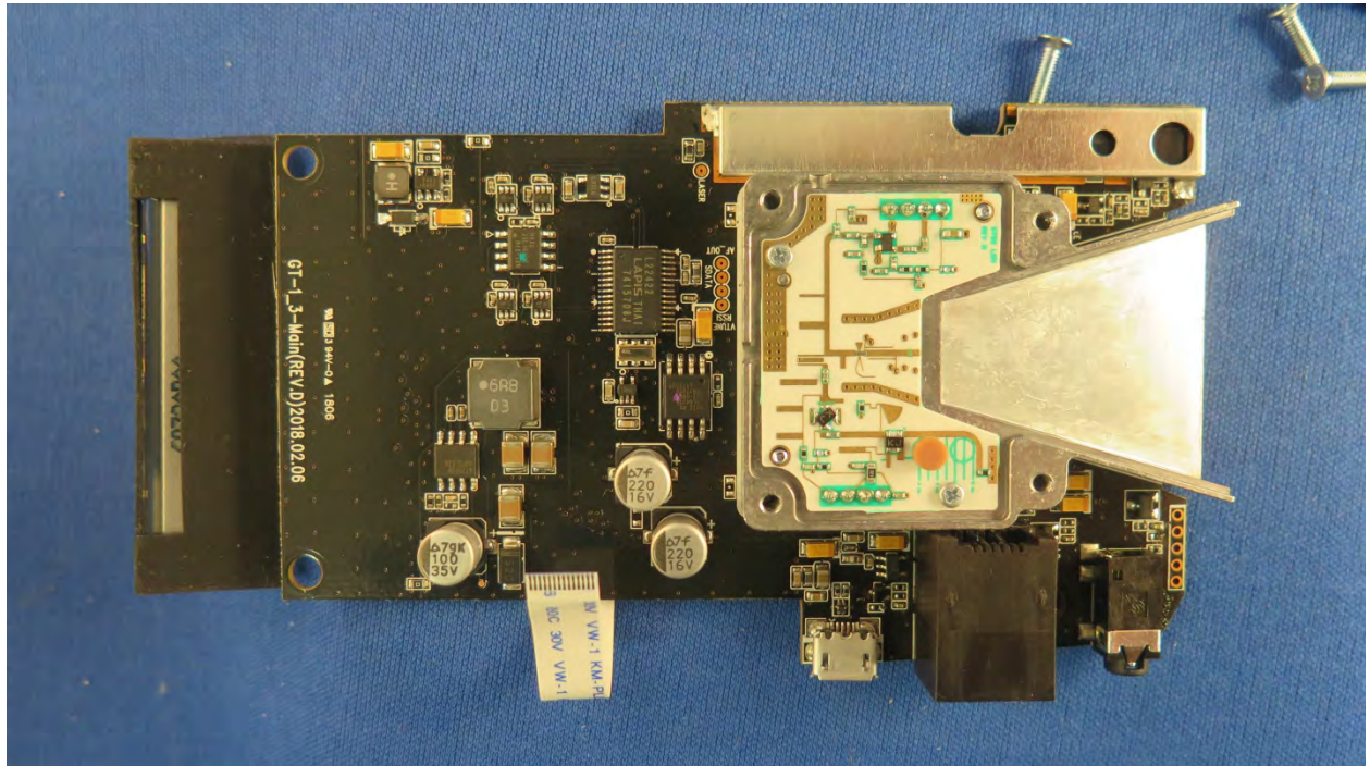
MAIN PCB – TOP VIEW – UPPER HORN REMOVED
