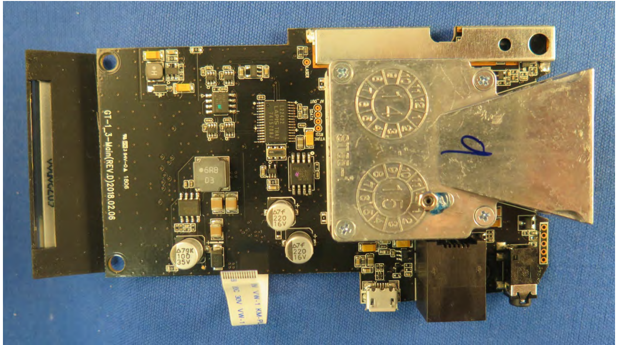
Main PCB TOP VIEW
