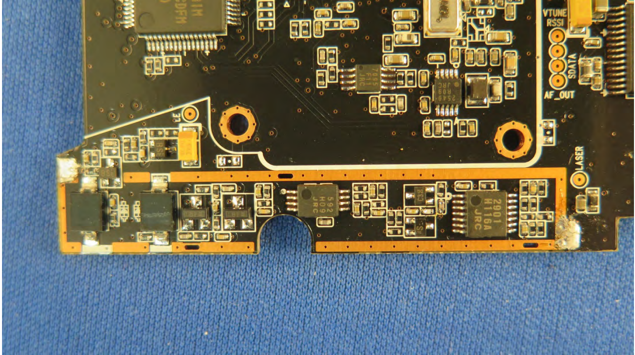
MAIN PCB – TOP VIEW LASER SHIELD REMOVED
