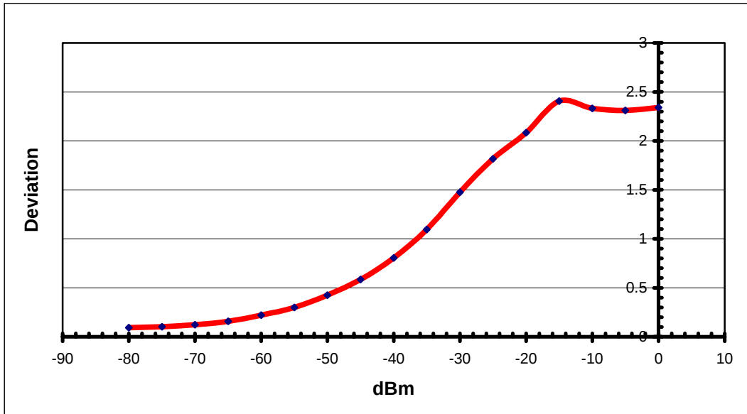
MODULATION LIMITING PLOT - 1000 Hz
