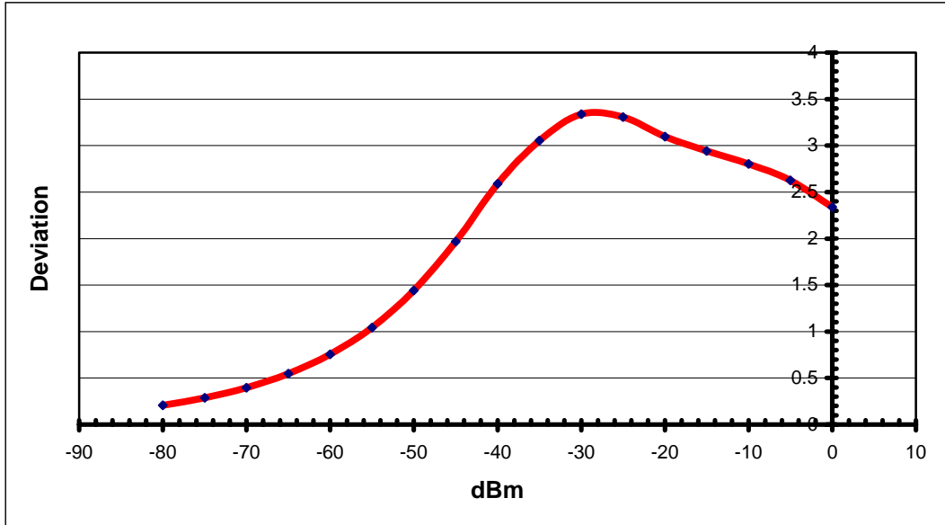
MODULATION LIMITING PLOT - 3000 Hz
