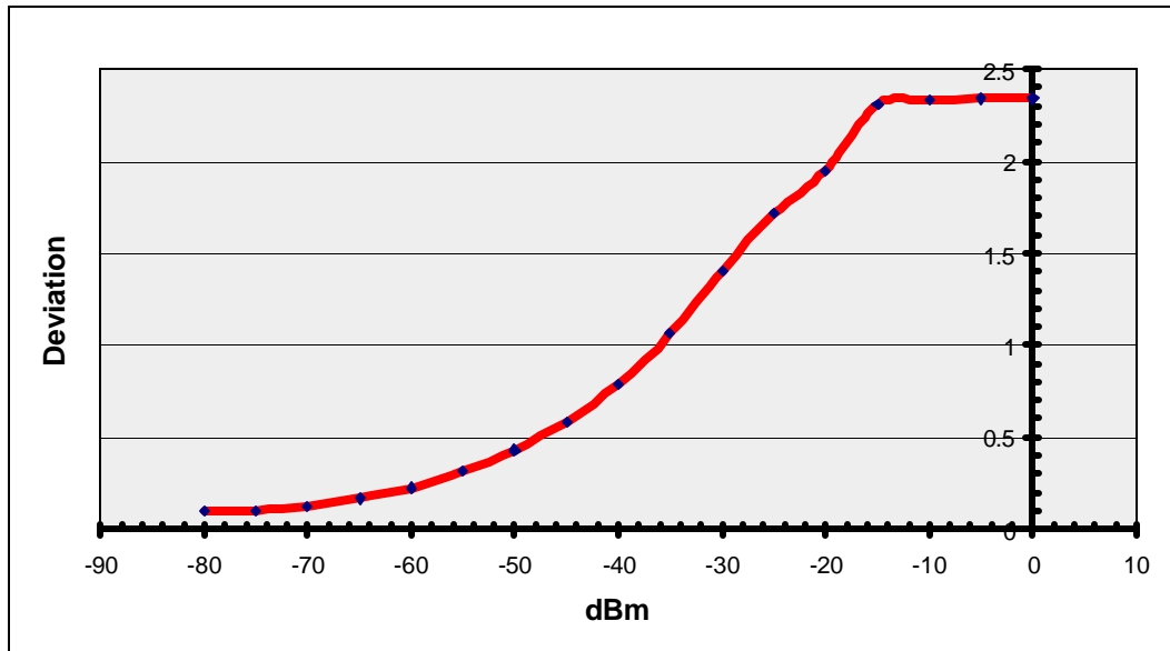
MODULATION LIMITING PLOT - 300 Hz
