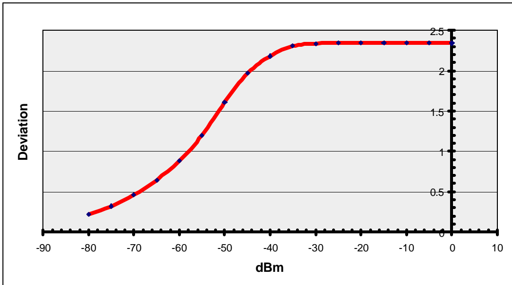
MODULATION LIMITING PLOT - 2500 Hz
