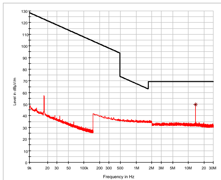
— Preview Result 1H-PK+ — FCC 15.209 mag (3 m) * Final_Result QPK
