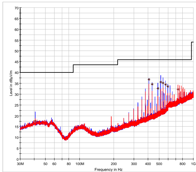
◇ Preview Result 1V-PK+ — FCC 15.209 * Final_Result QPK — Final_Result AVG — Preview Result 1H-PK+
