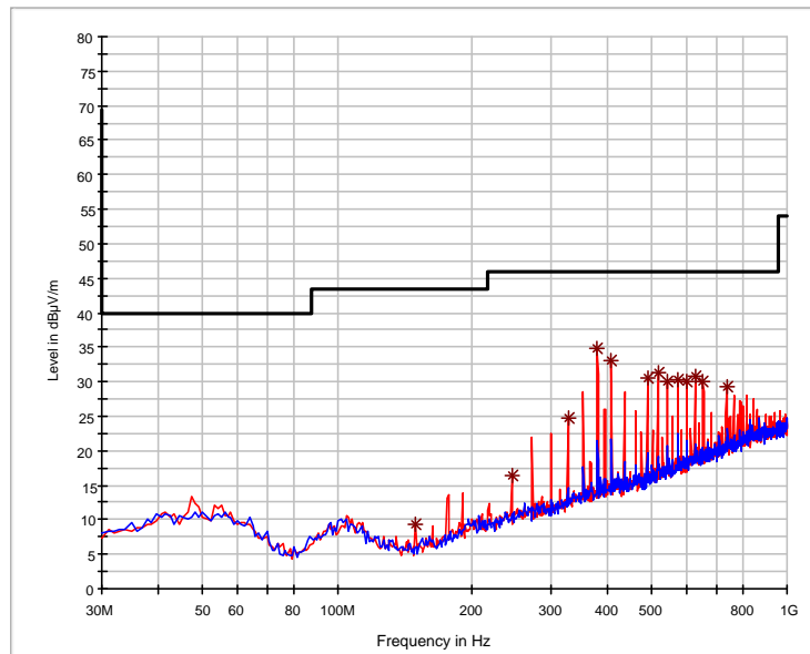
Preview Result 1H-PK+ Preview Result 1V-PK+ FCC 15.209 * Final_Result PK+
