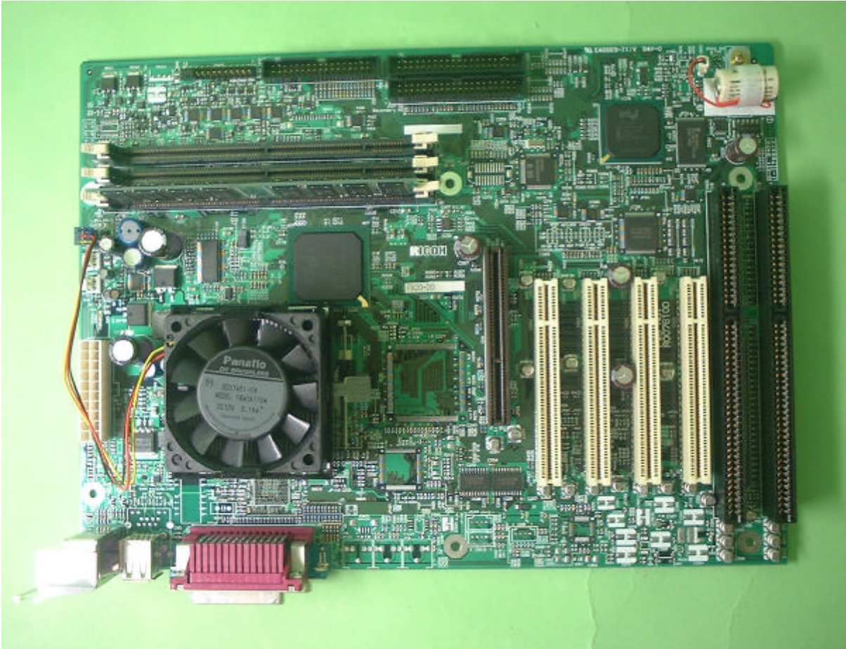
CPU<Top view>
