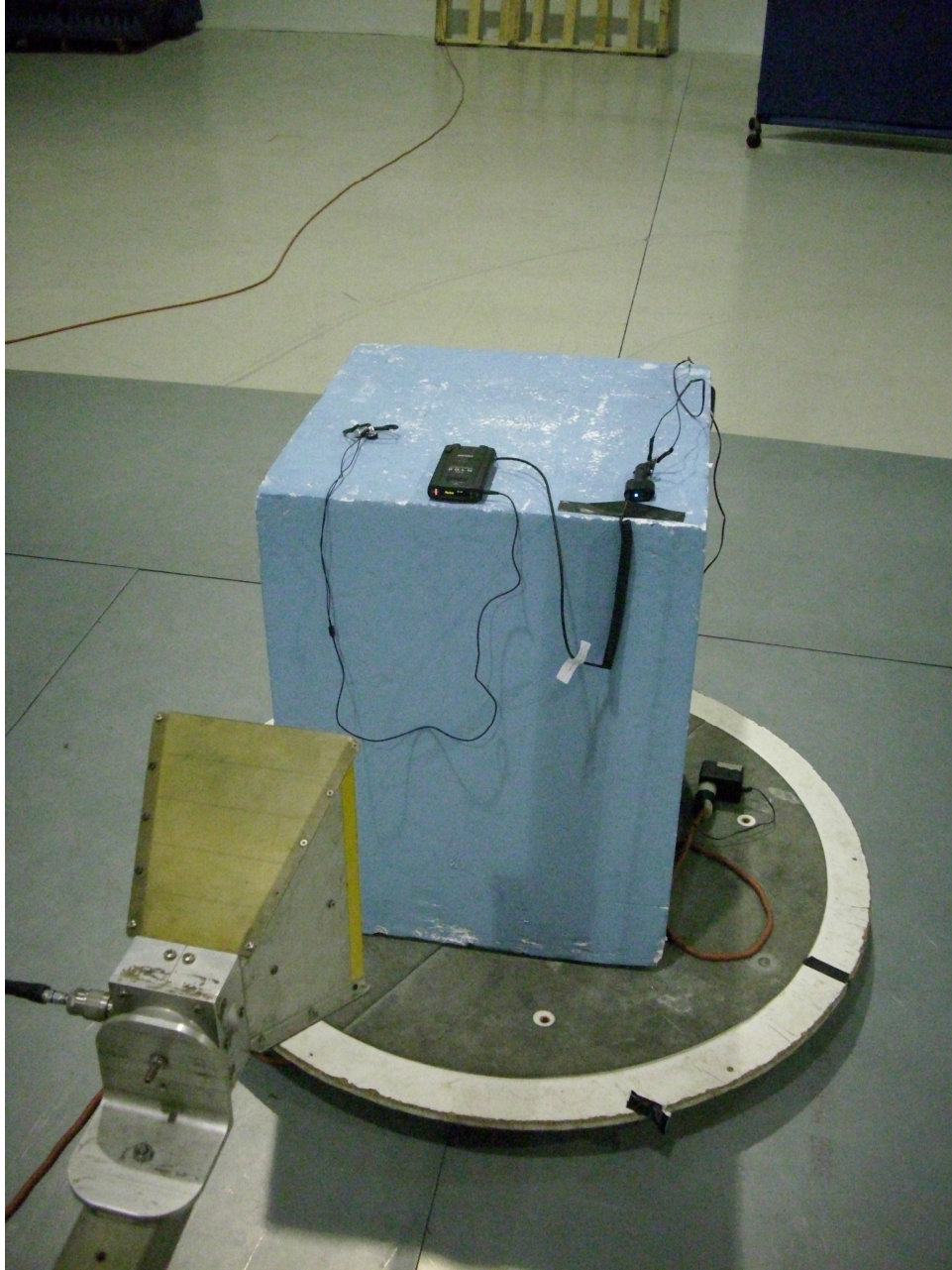
Radiated Emissions at OATS
