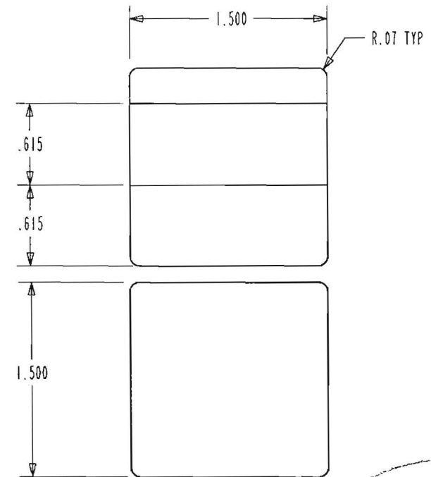
OVERALL AND FACE SPLIT DIMS (SCALE 1:1)
