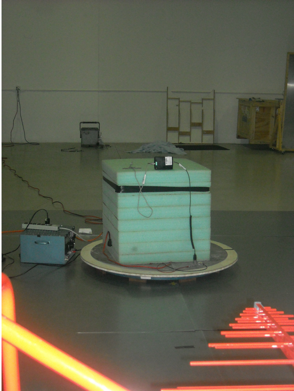
Radiated Emissions Below 1GHz in OATS
