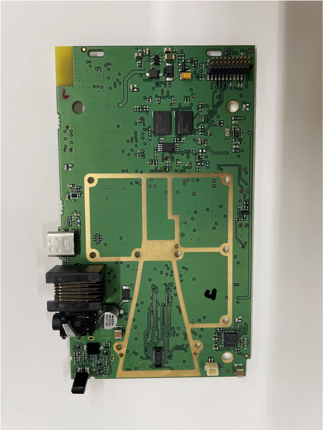
Main Board
