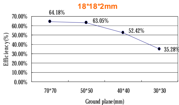
Efficiency vs. ground plane
