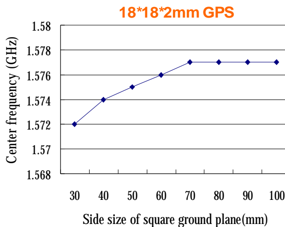
Frequency vs. ground plane
