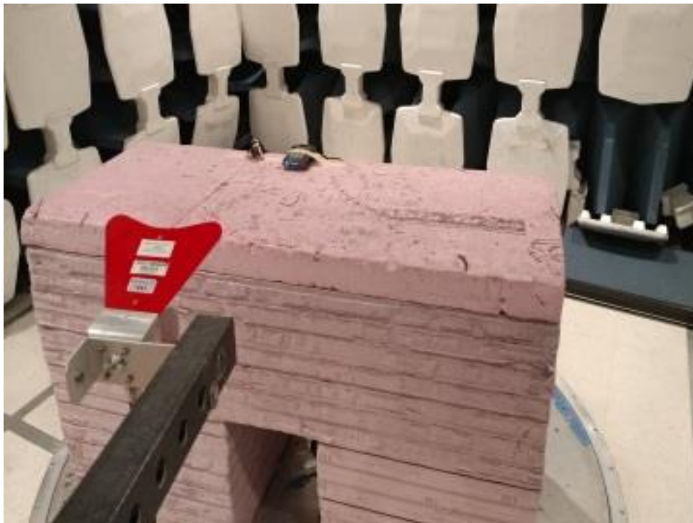
Radiated Emissions Setup – 11.7 to 12.2 GHz (front)
