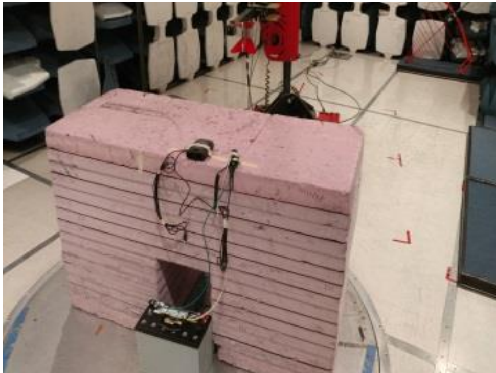
Radiated Emissions Setup – 11.7 to 12.2 GHz (rear)
