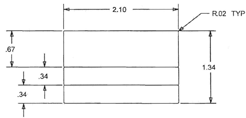
OVERALL AND FACE SPLIT DIMS (SCALE 1:1)
