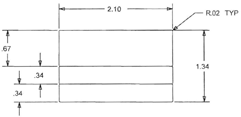
OVERALL AND FACE SPLIT DIMS (SCALE 1:1)
