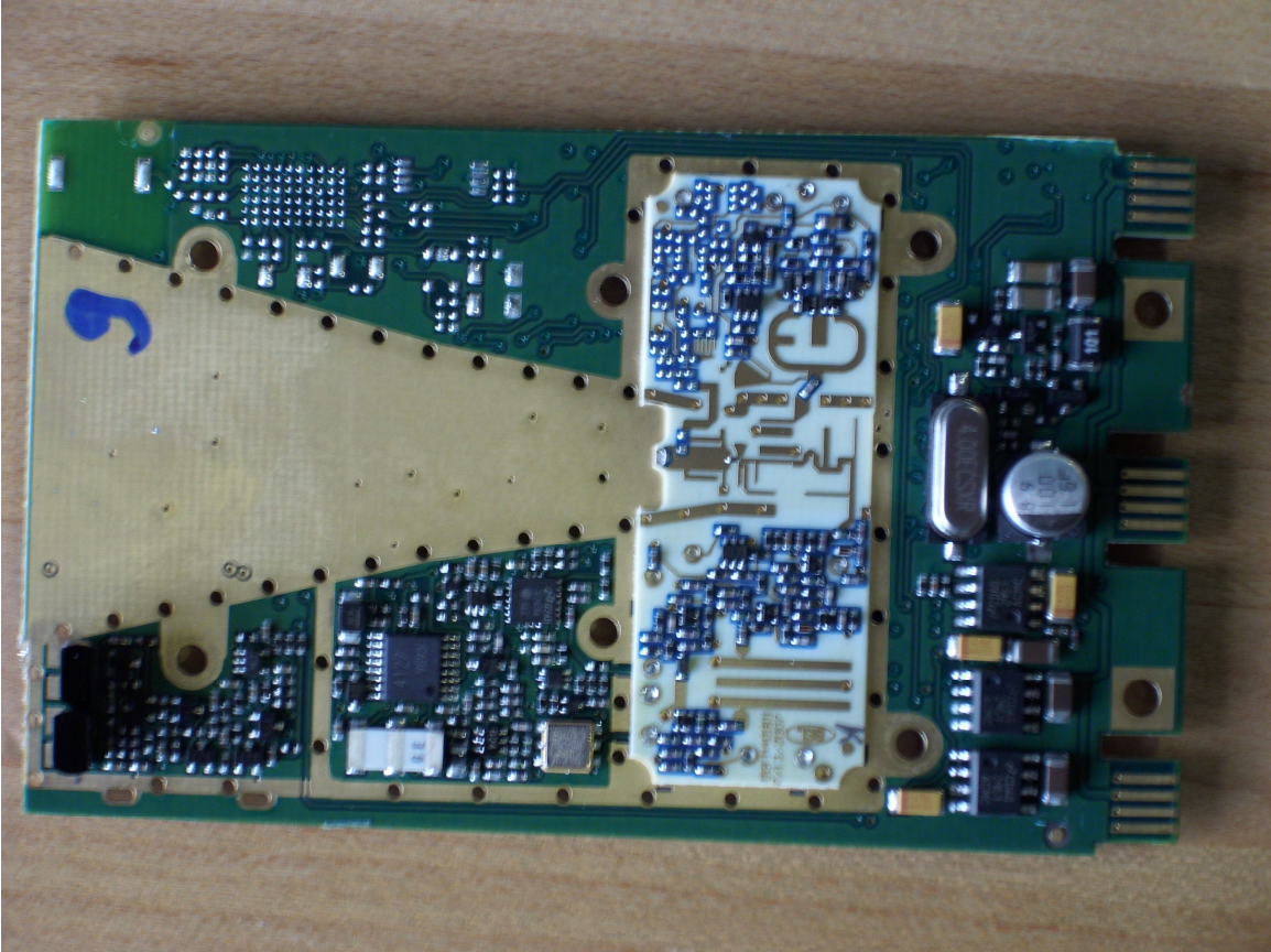
Top View without Shield
