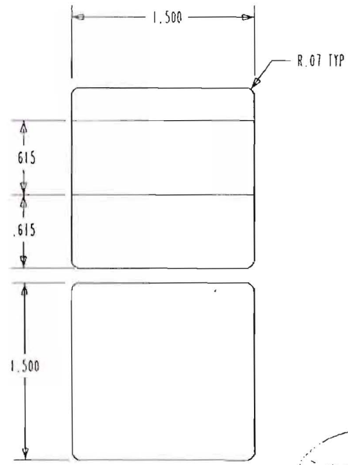
OVERALL AND FACE SPLIT DIMS (SCALE 1:1)
