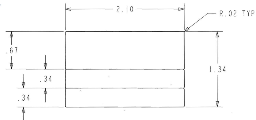
OVERALL AND FACE SPLIT DIMS (SCALE 1:1)
