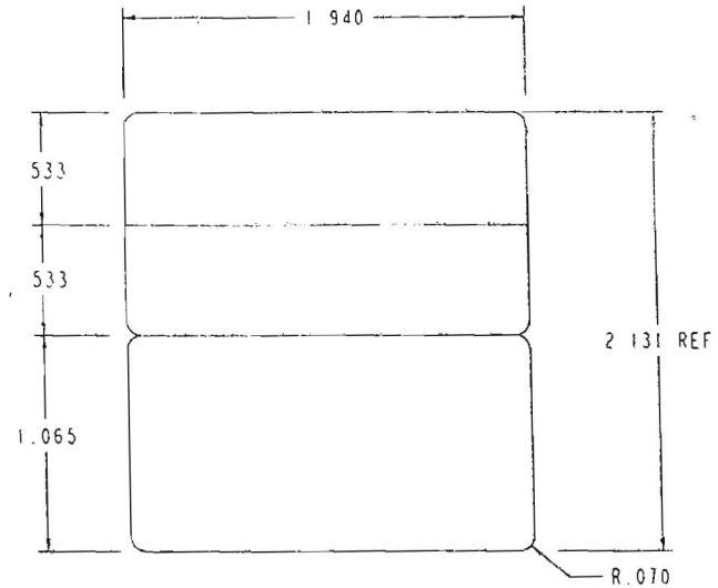
OVERALL AND FACE SPLIT DIMS (SCALE 1:1)
