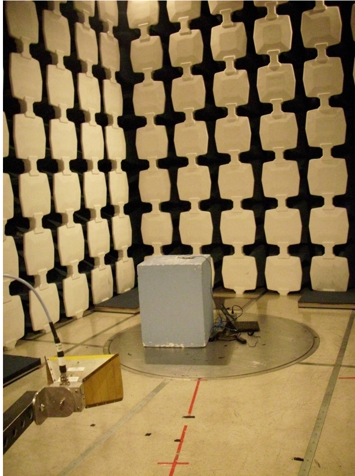
Radiated Emissions Measurements – Above 1GHz – Anechoic Chamber
