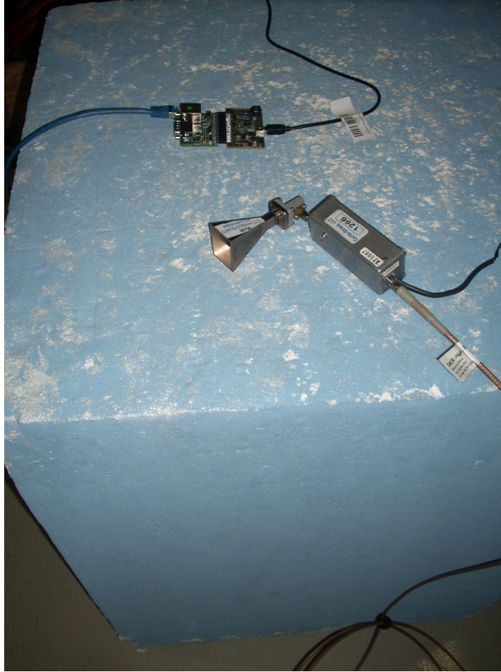
Radiated Emission Measurements 18-25GHz
