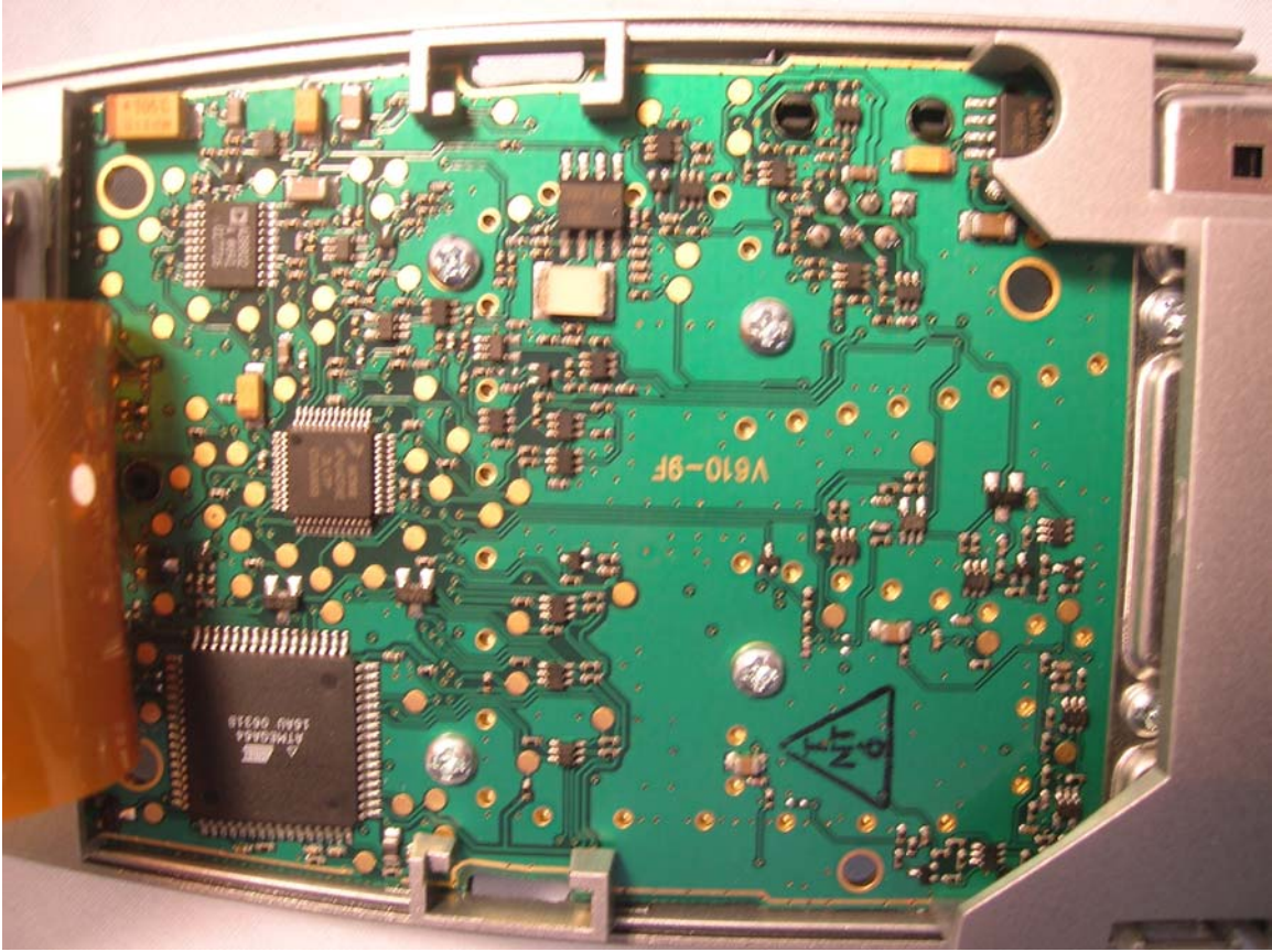
Under daughter card picture 2
