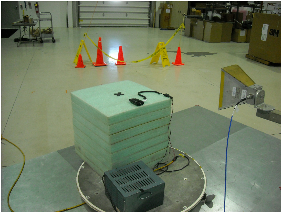
Radiated EMI
