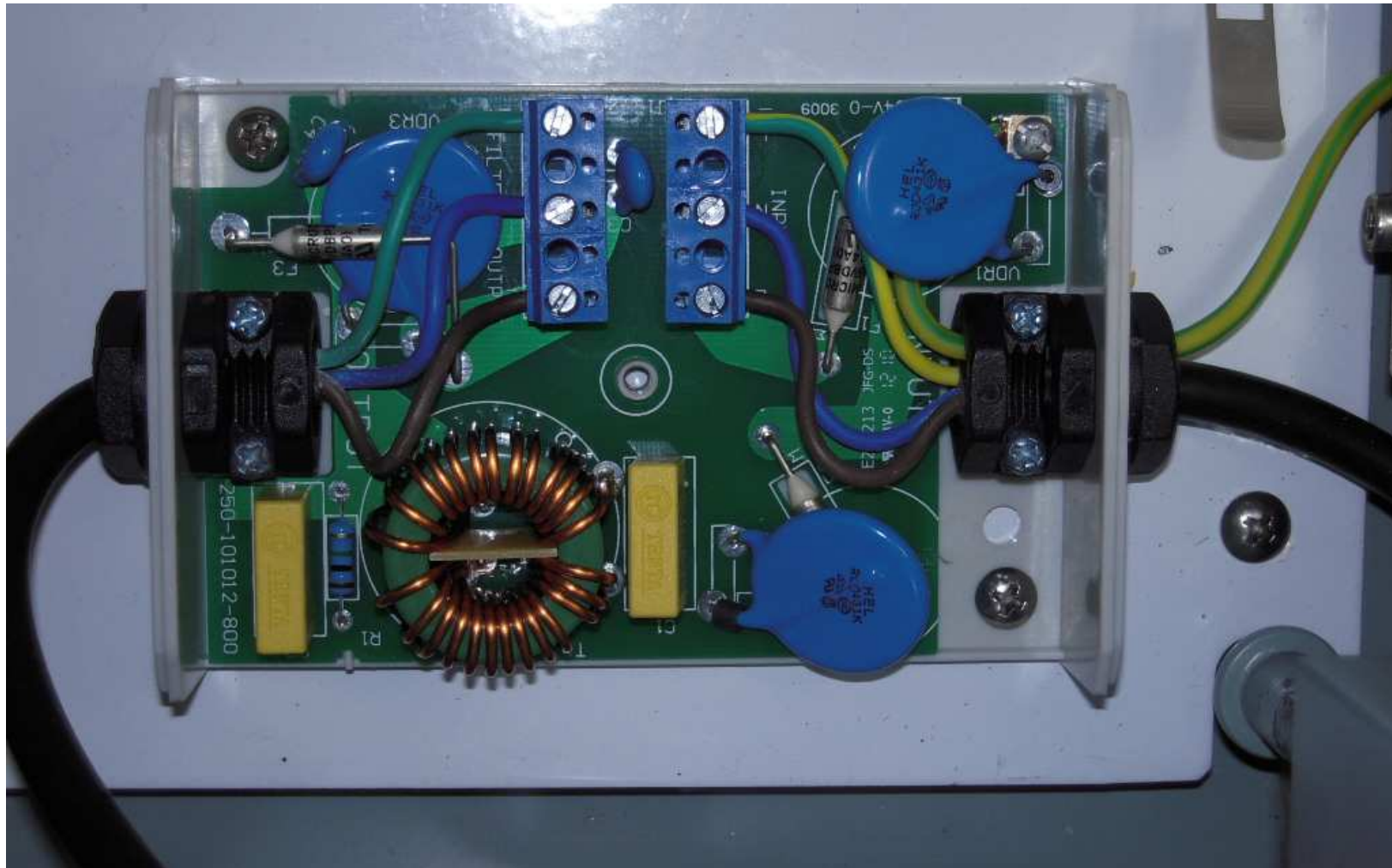
PHOTOGRAPH OF THE PRODUCT (Surge Filter) INNER CIRCUIT TOP VIEW
