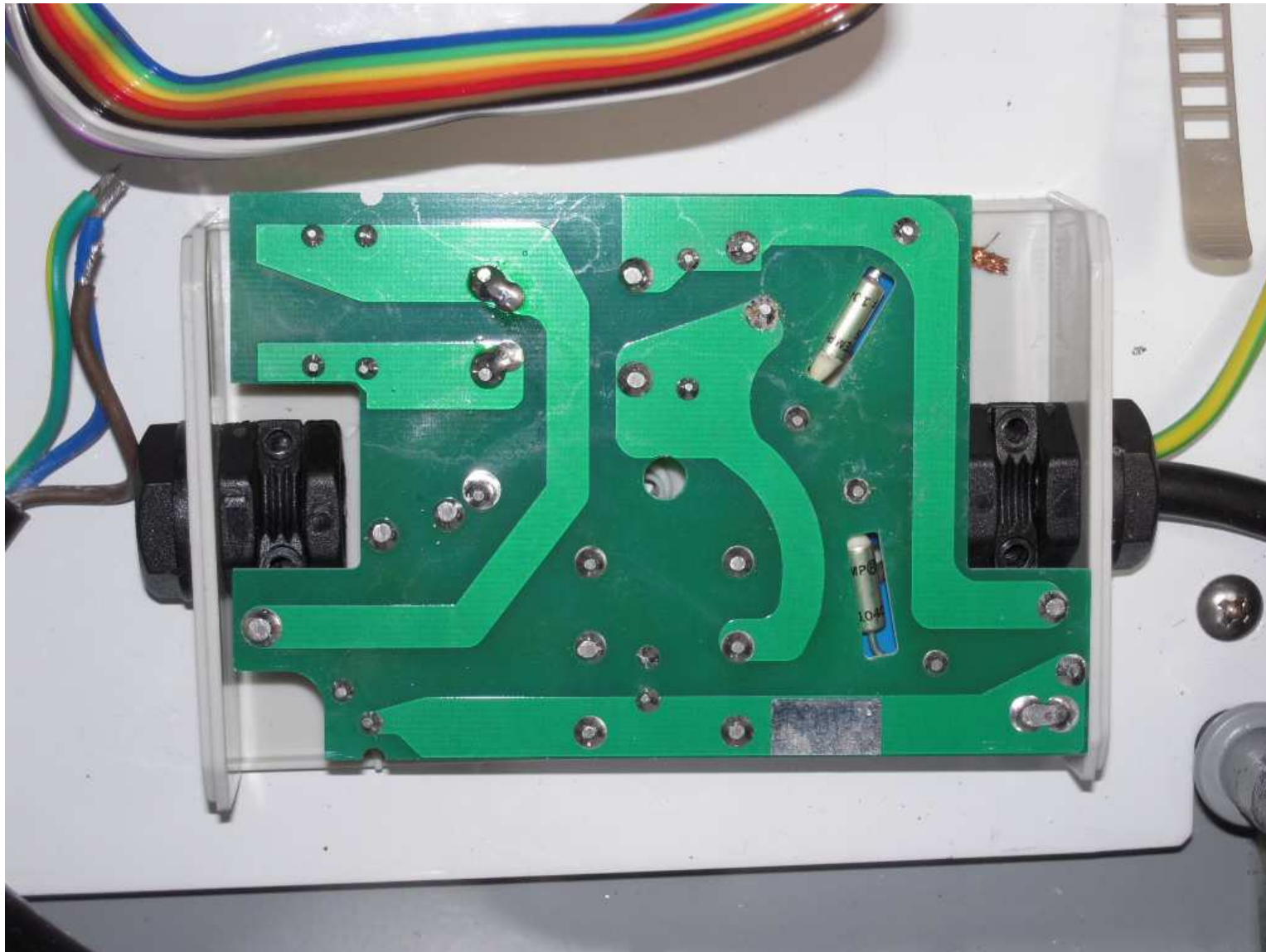
PHOTOGRAPH OF THE PRODUCT (Surge Filter) INNER CIRCUIT BOTTOM VIEW
