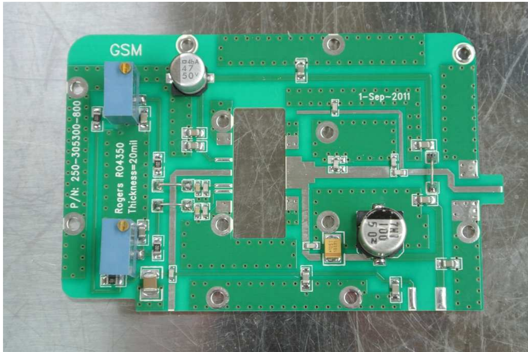
PHOTOGRAPH OF THE PRODUCT (CM850) INNER CIRCUIT TOP VIEW
