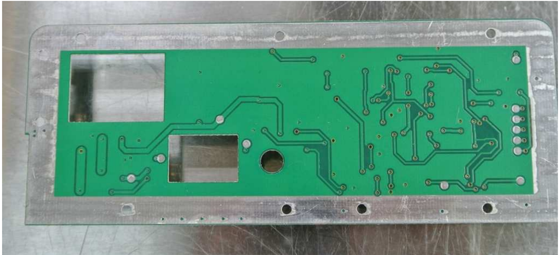
PHOTOGRAPH OF THE PRODUCT (CM851) INNER CIRCUIT BOTTOM VIEW
