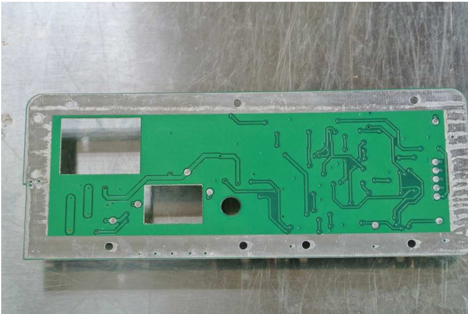
PHOTOGRAPH OF THE PRODUCT (CM850) INNER CIRCUIT BOTTOM VIEW
