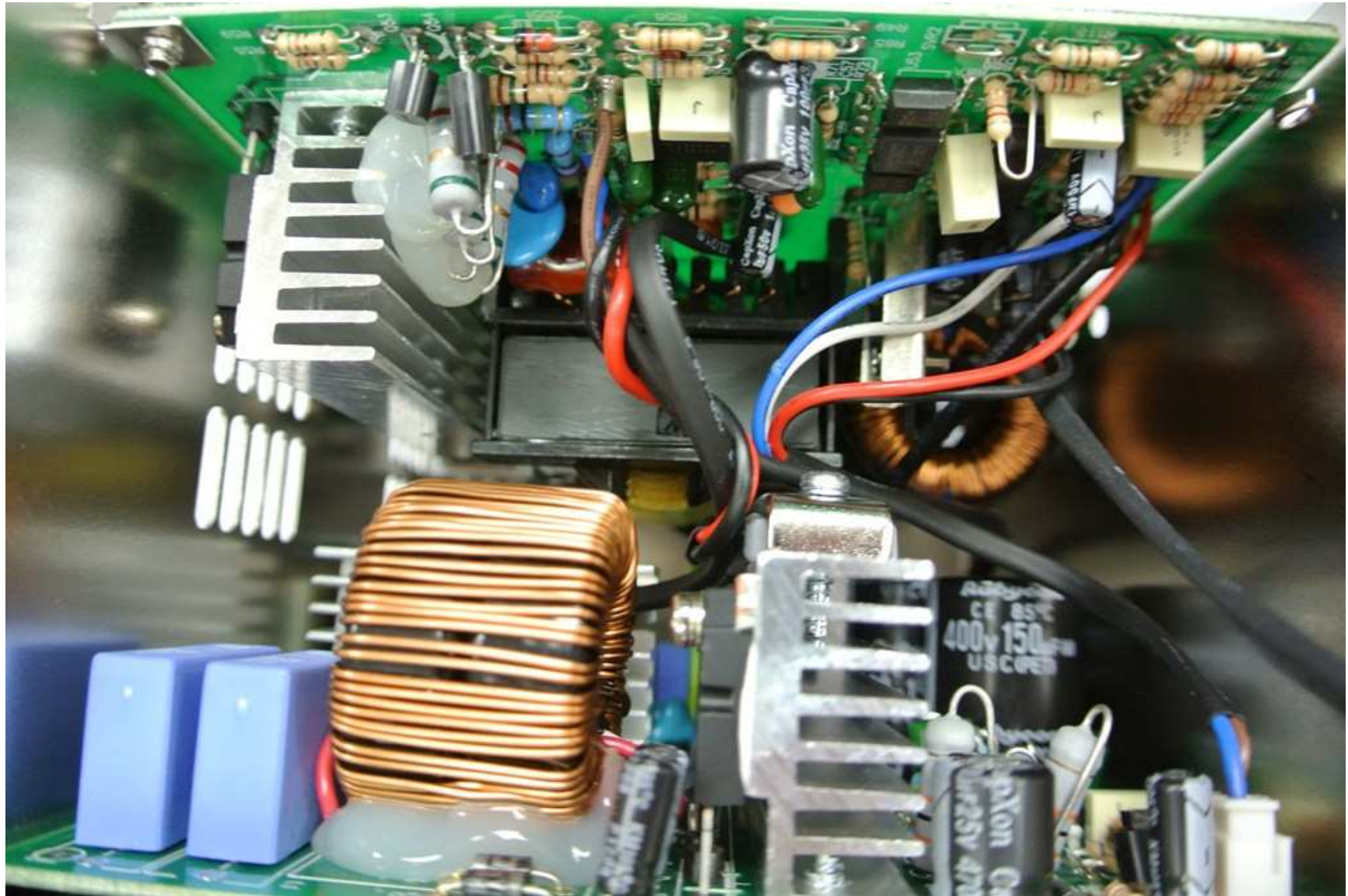
PHOTOGRAPH OF THE PRODUCT ( Power Supply )
