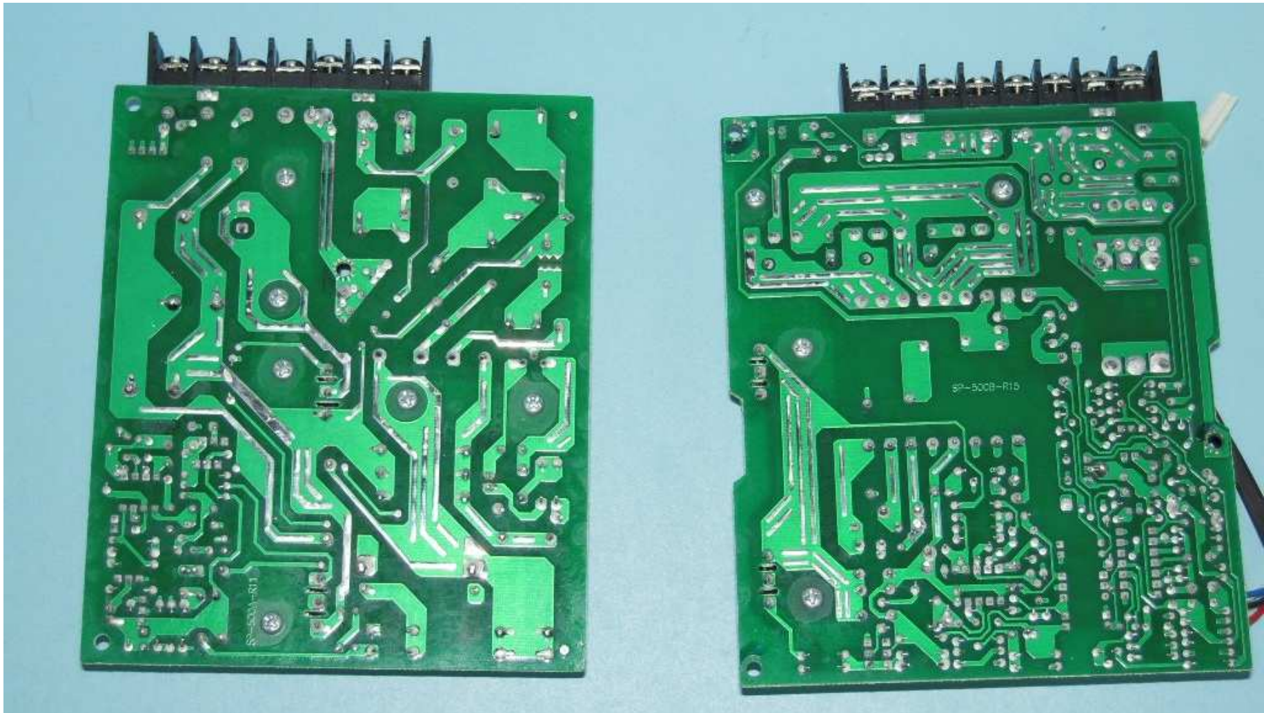
PHOTOGRAPH OF THE PRODUCT (Power Supply) INNER CIRCUIT BOTTOM VIEW
