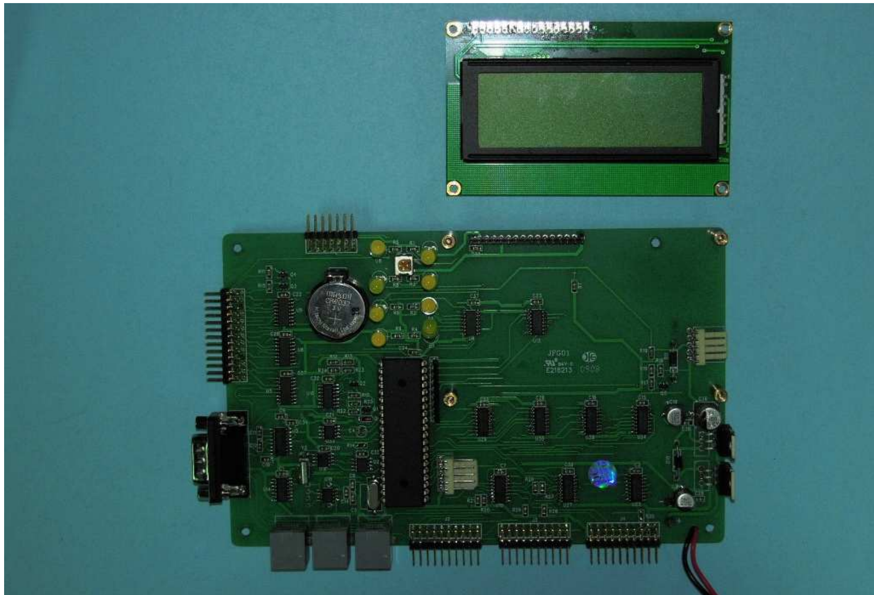
PHOTOGRAPH OF THE PRODUCT (Controller) INNER CIRCUIT TOP VIEW
