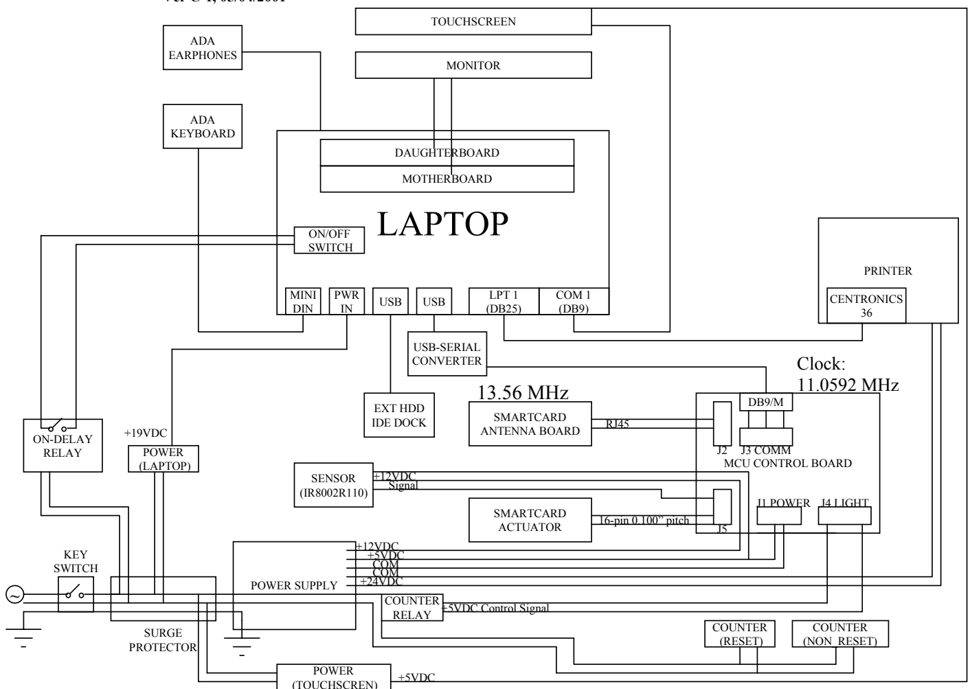
VoteTrakker Electrical Schematic
