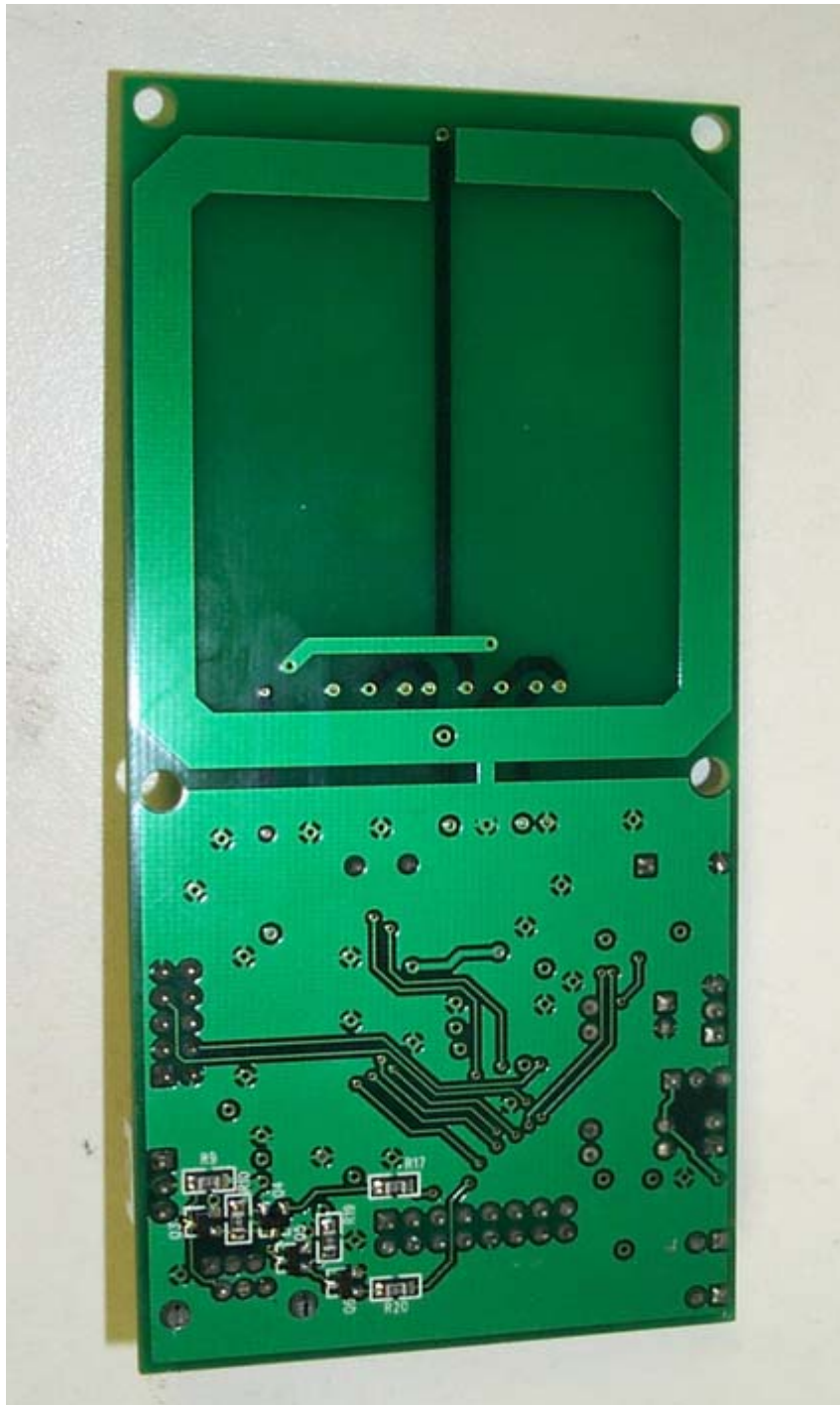
Card Reader Foil Side
