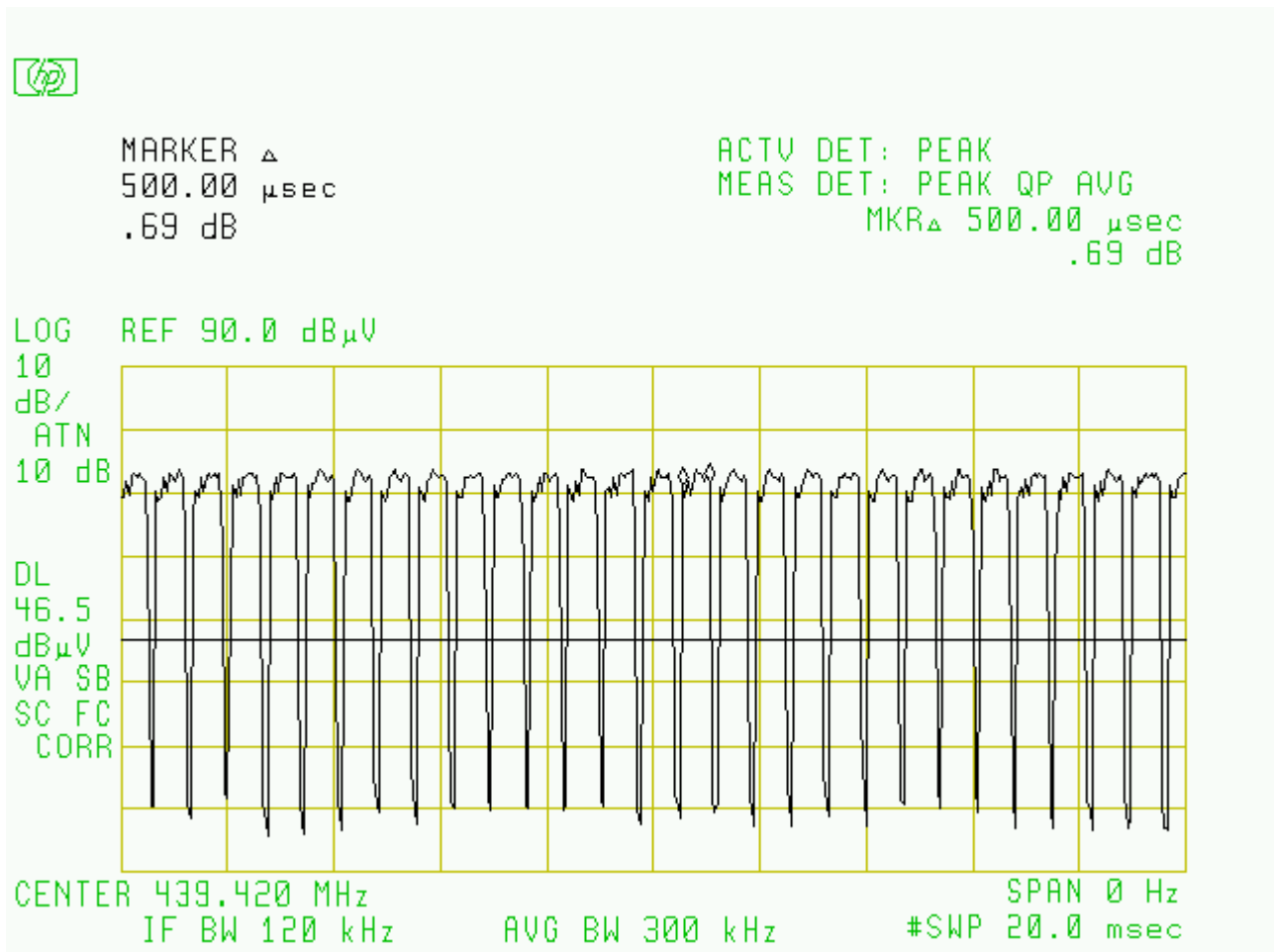
Figure 6.2 Pulse Train Timing
