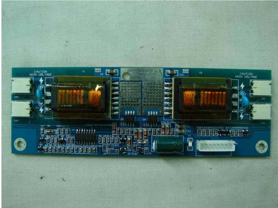
Inverter (Rear)
