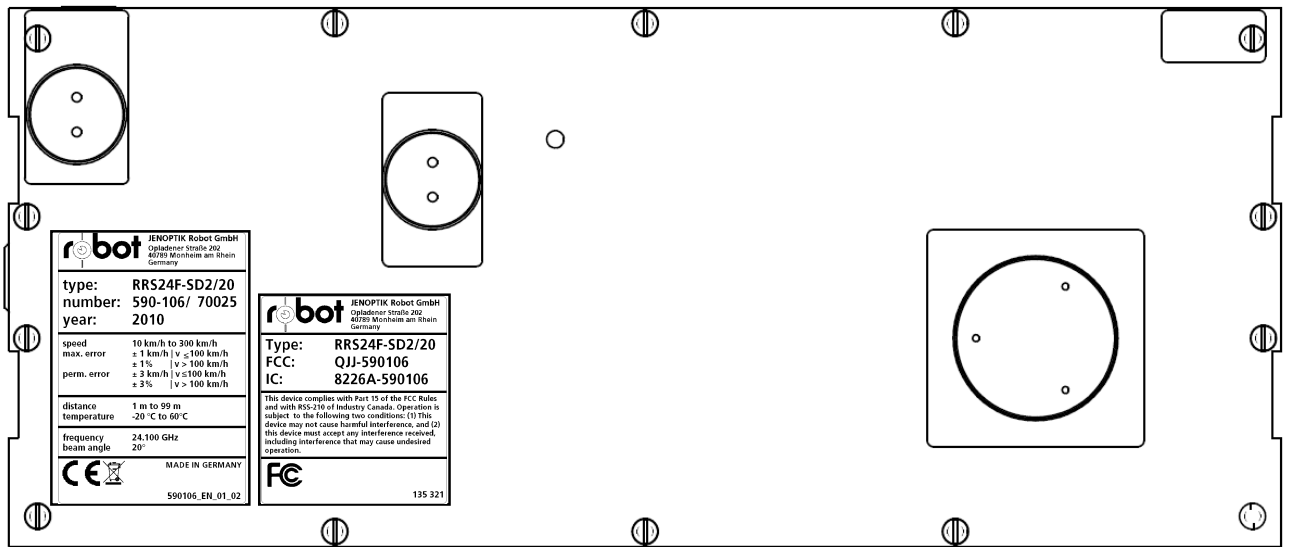
Figure 1 - Label placement on rear of RRS24F-SD2/20
