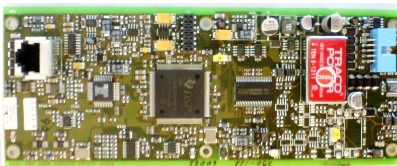
Picture 3: Signal processing board (backside)
