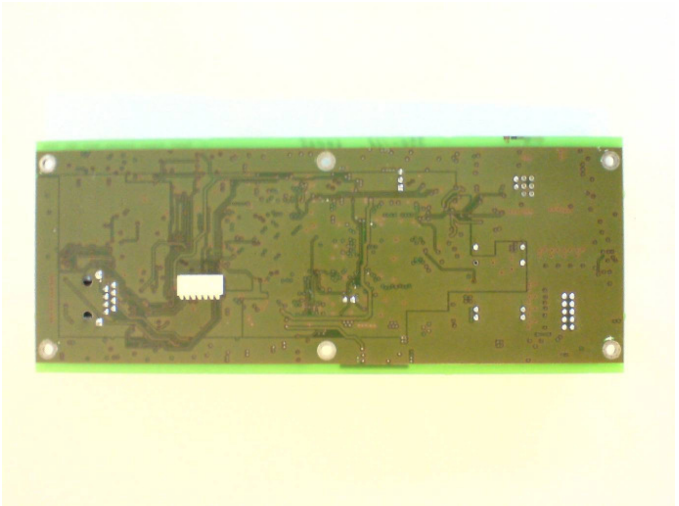
EUT mainboard rear view
