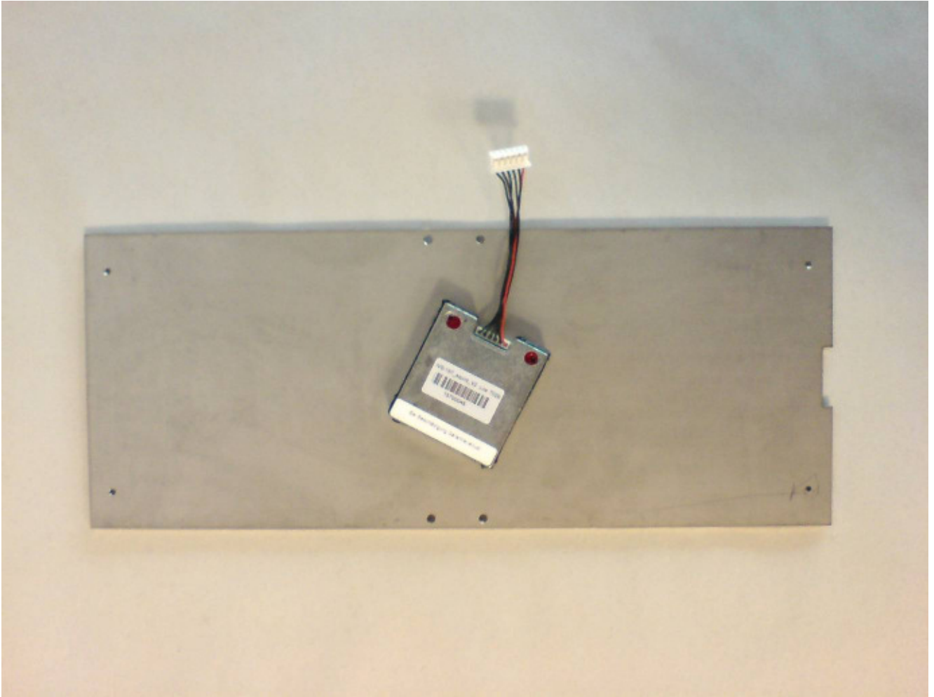
EUT microwave unit with antenna field (rear view)
