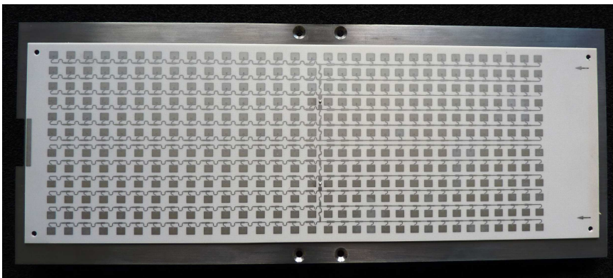
Picture 2: Radar Frontend (frontside)
