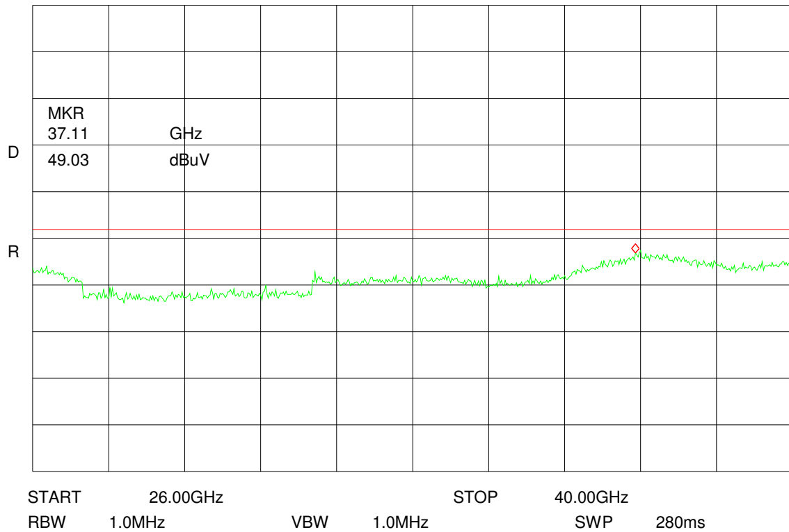
*ATTEN 0dB MKR 49.03dBuV RL 102.2dBuV 10dB/ 37.11GHz
