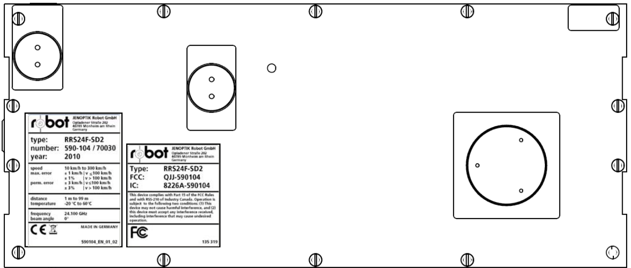
Figure 1 - Label placement on rear of RRS24F-SD2
