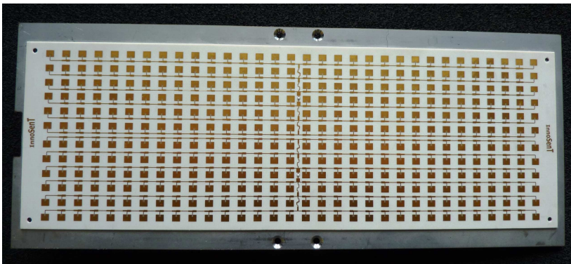
Picture 2: Radar Frontend (frontside)
