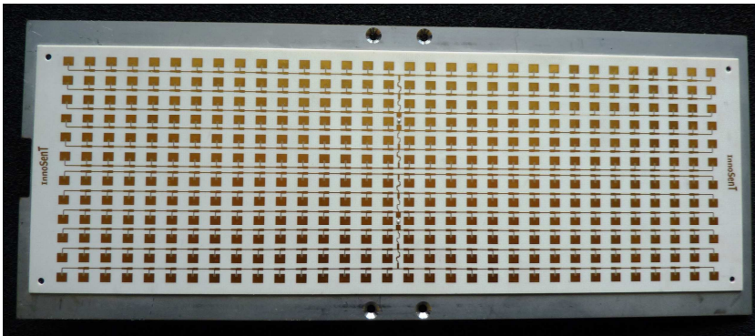
Picture 2: Radar Frontend (frontside)
