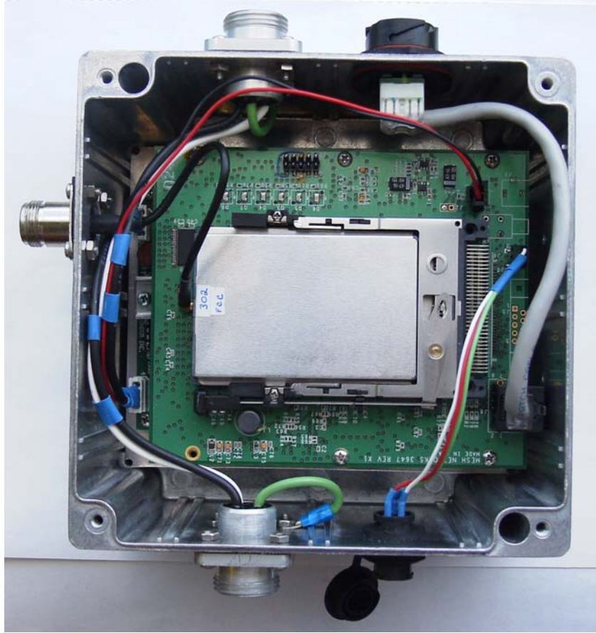
IAP6300 Opened Box
