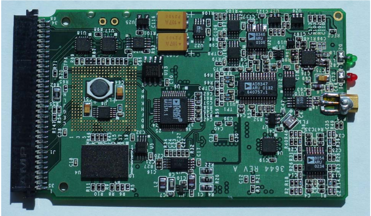
IAP6300 PCMCIA Bottom Side
