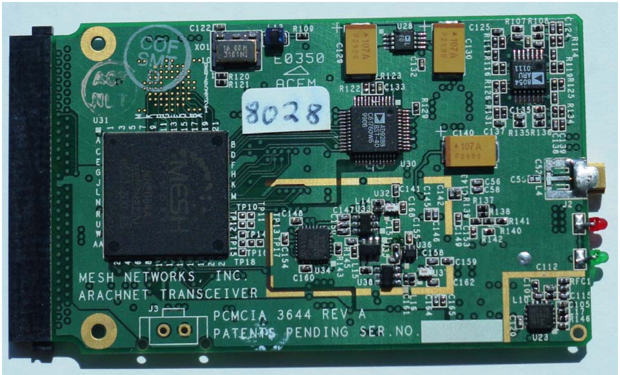
IAP6300 PCMCIA Top Side
