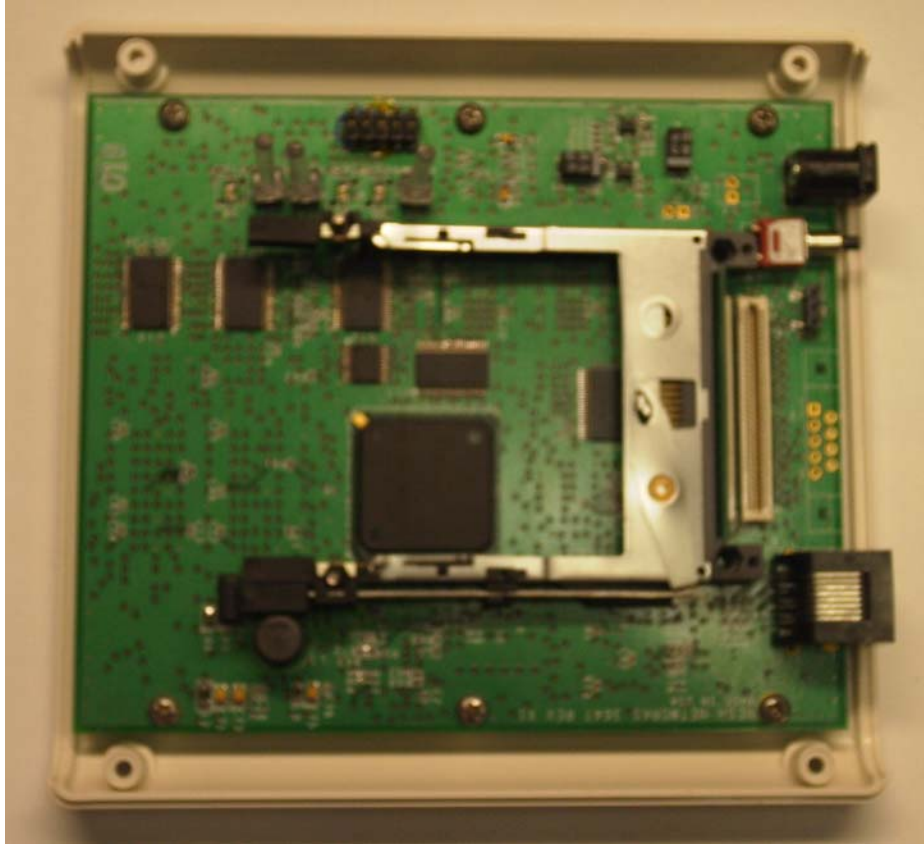
AP400 Single Board Computer in Bottom Housing View
