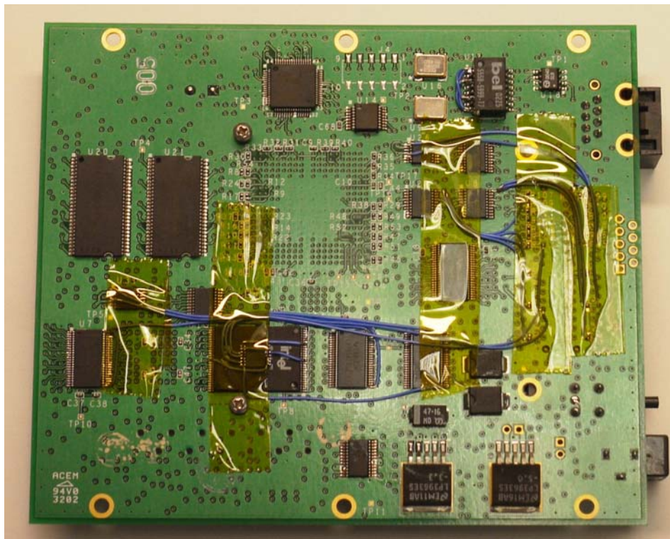
AP400 Single Board Computer Bottom Side View
