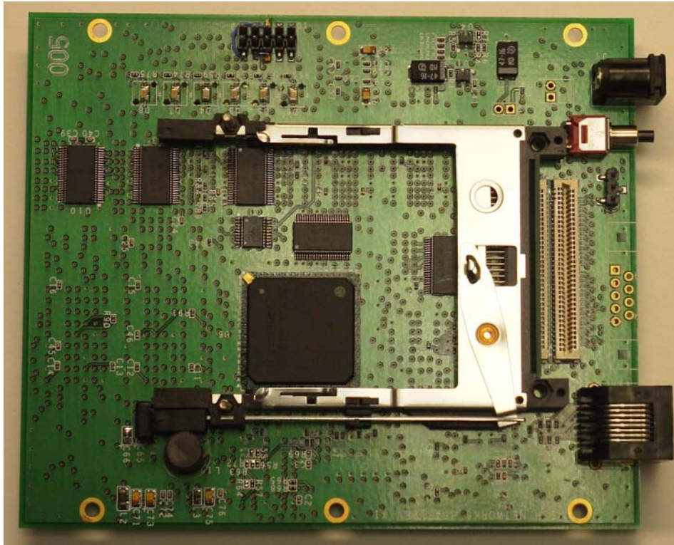
AP400 Single Board Computer Top Side View
