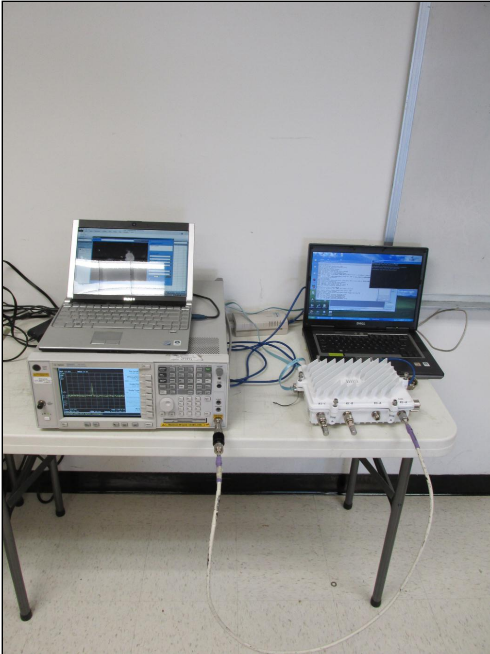
Photograph 1. Conducted Power, Test Setup
