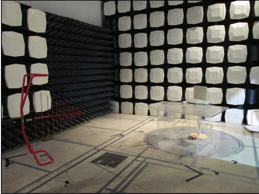
Photograph 2. Radiated Emissions, Test Setup, Below 1 GHz
