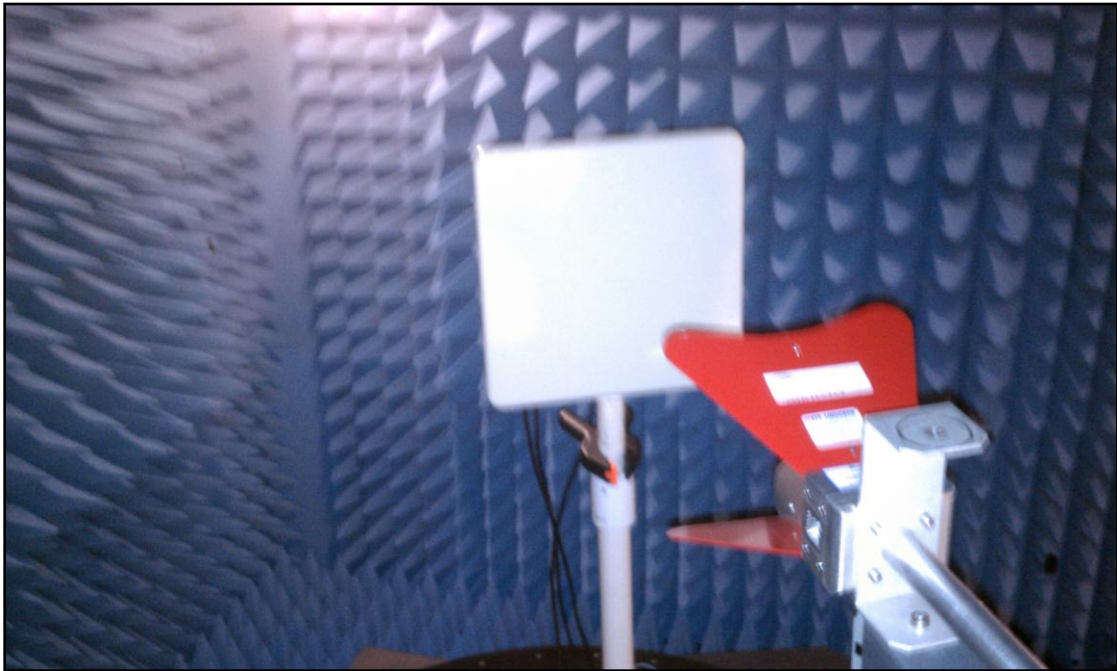
Photograph 3. Radiated Emissions, Test Setup, Panel Antenna
