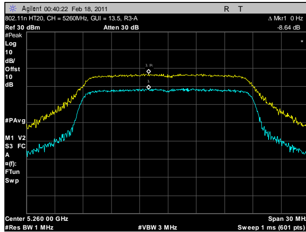
Plot 139. Peak Excursion Ratio, 802.11n HT20, 5260 MHz, R3-A
