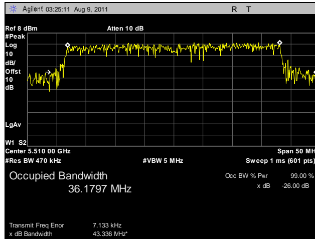
Plot 58. 26 dB Occupied Bandwidth, 802.11n HT40, 5510 MHz, R3-A
