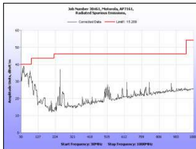
Plot 201. Radiated Spurious Emissions, 30 MHz – 1 GHz, 802.11n HT20, 5320 MHz
