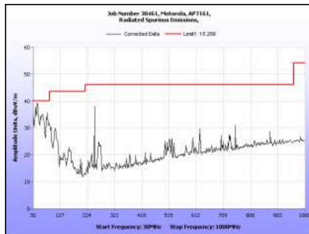
Plot 197. Radiated Spurious Emissions, 30 MHz – 1 GHz, 802.11n HT20, 5300 MHz
