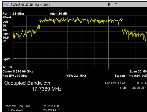
Plot 35. 26 dB Occupied Bandwidth, 802.11n HT20, 5320 MHz, R3-B
