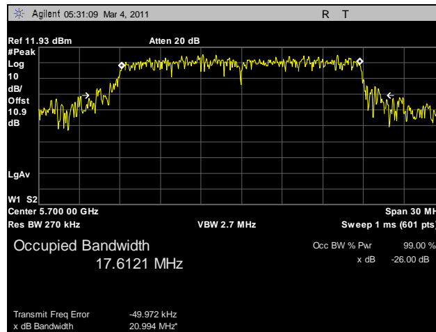
Plot 46. 26 dB Occupied Bandwidth, 802.11n HT20, 5700 MHz, R3-A
