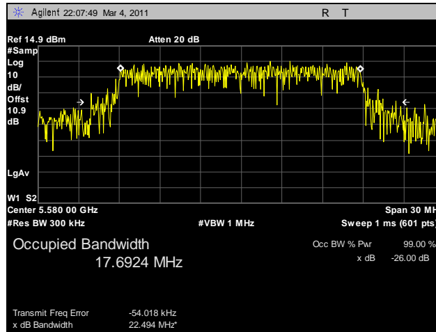
Plot 100. 99% Occupied Bandwidth, 802.11n HT20, 5580 MHz, R3-A
