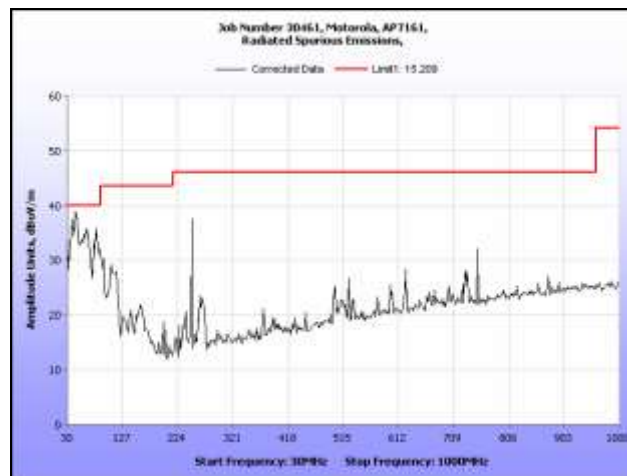
Plot 221. Radiated Spurious Emissions, 30 MHz – 1 GHz, 802.11n HT40, 5300 MHz
