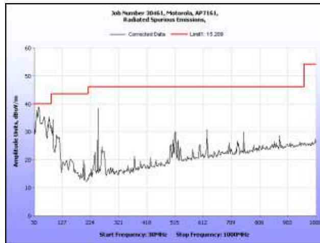
Plot 173. Radiated Spurious Emissions, 30 MHz – 1 GHz, 802.11a, 5300 MHz
