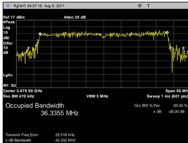
Plot 65. 26 dB Occupied Bandwidth, 802.11n HT40, 5670 MHz, R3-B
