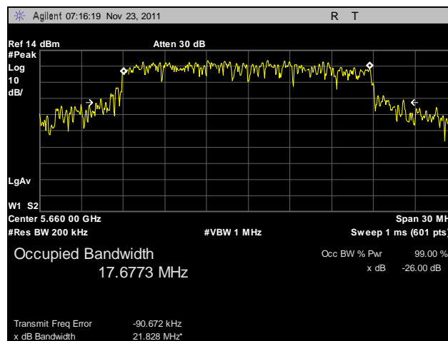
Plot 45. 26 dB Occupied Bandwidth, 802.11n HT20, 5660 MHz, R3-C
