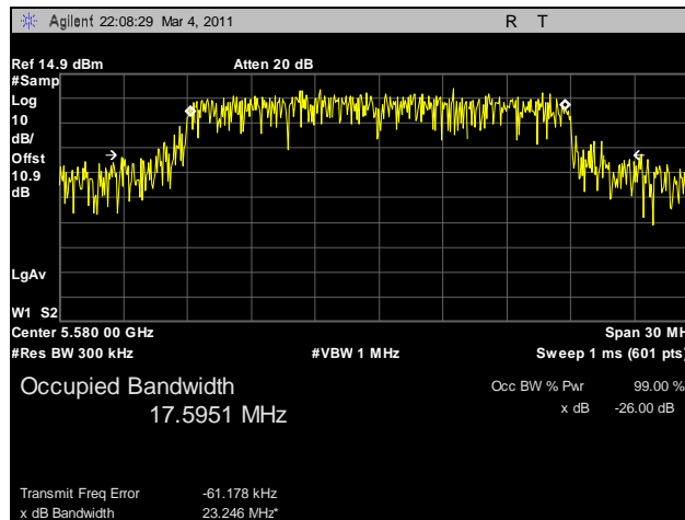
Plot 102. 99% Occupied Bandwidth, 802.11n HT20, 5580 MHz, R3-C
