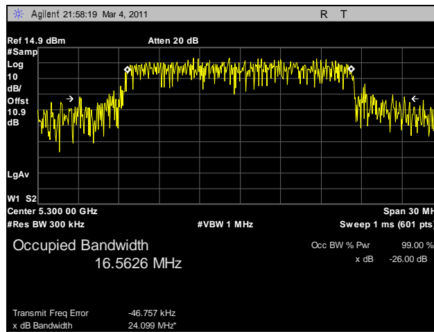
Plot 74. 99% Occupied Bandwidth, 802.11a, 5300 MHz, R3-B
