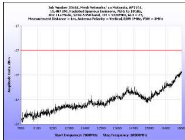
Plot 179. Radiated Spurious Emissions, 7 GHz – 18 GHz, 802.11a, 5320 MHz
