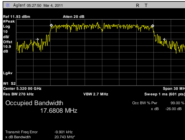
Plot 34. 26 dB Occupied Bandwidth, 802.11n HT20, 5320 MHz, R3-A
