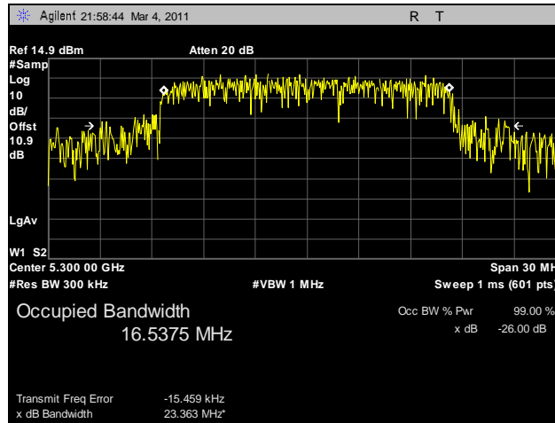
Plot 73. 99% Occupied Bandwidth, 802.11a, 5300 MHz, R3-A
