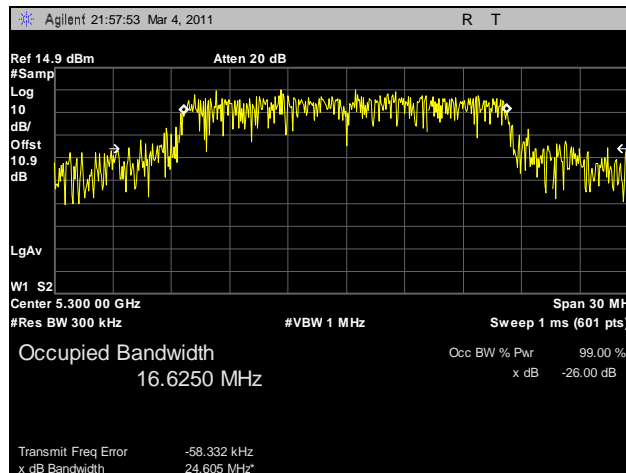
Plot 75. 99% Occupied Bandwidth, 802.11a, 5300 MHz, R3-C
