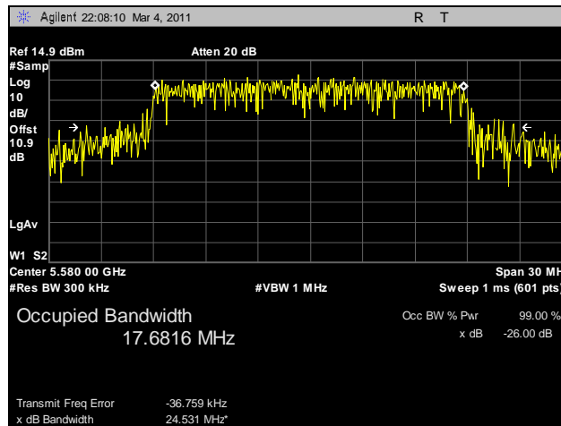
Plot 101. 99% Occupied Bandwidth, 802.11n HT20, 5580 MHz, R3-B
