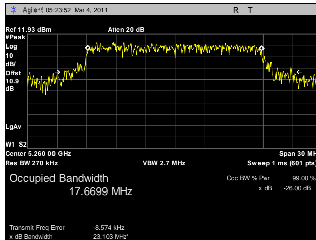
Plot 30. 26 dB Occupied Bandwidth, 802.11n HT20, 5260 MHz, R3-C
