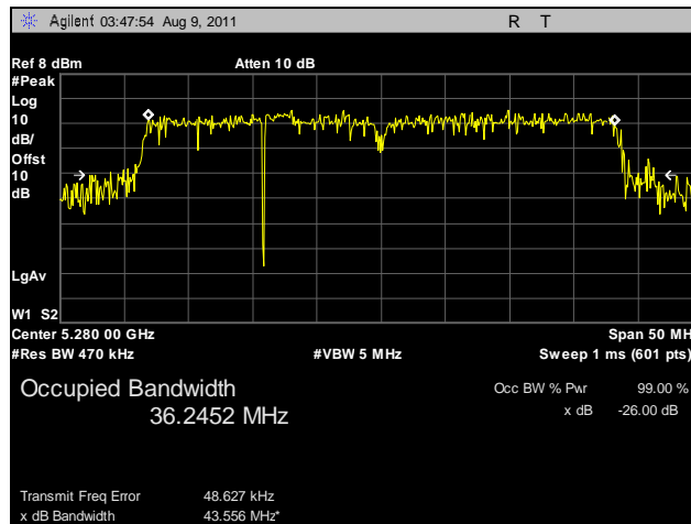
Plot 50. 26 dB Occupied Bandwidth, 802.11n HT40, 5280 MHz, R3-B
