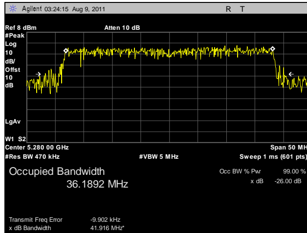
Plot 49. 26 dB Occupied Bandwidth, 802.11n HT40, 5280 MHz, R3-A
