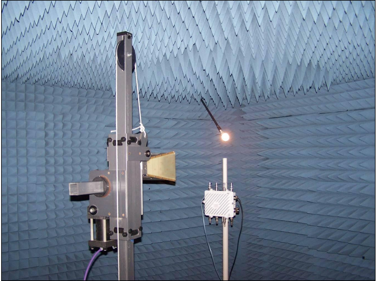
Photograph 3. Radiated Emission Spurious Test Setup
