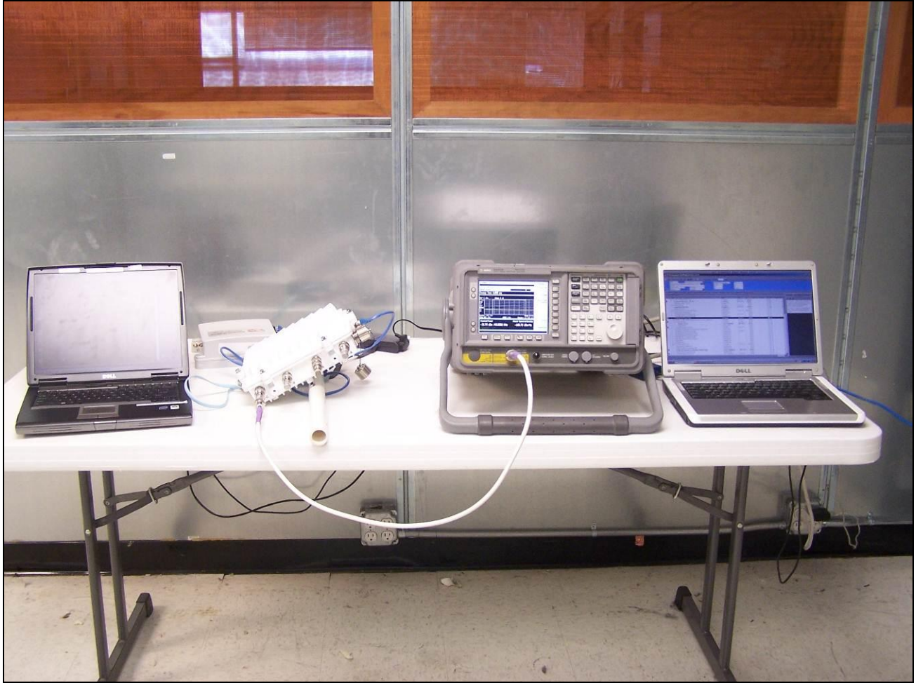
Photograph 2. Peak Power Spectral Density, Test Setup
