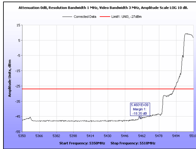
Plot 106. EIRP, 5500 MHz, 802.11a, Band Edge
