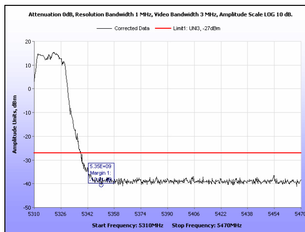
Plot 111. EIRP, 5320 MHz, 802.11n 20 MHz, Band Edge
