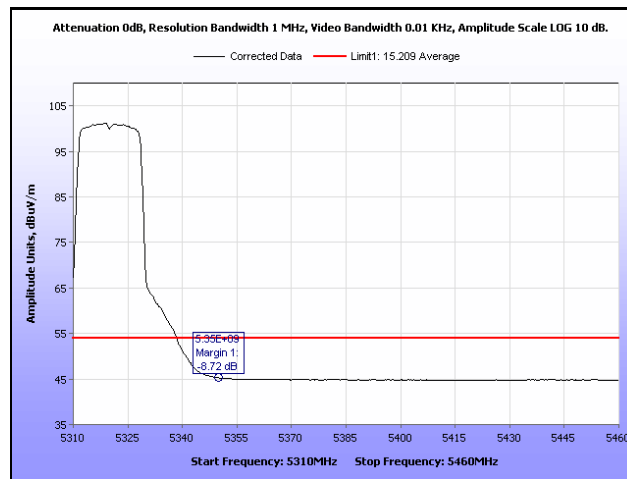
Plot 117. Restricted Band, 802.11a, 5320 MHz, Average
