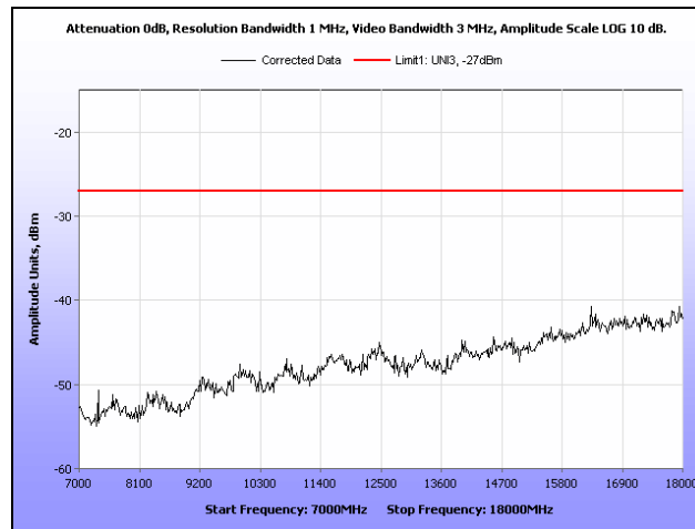
Plot 83. Radiated Spurious Emissions, 5510 MHz, 802.11n 40 MHz, 7 GHz – 18 GHz
