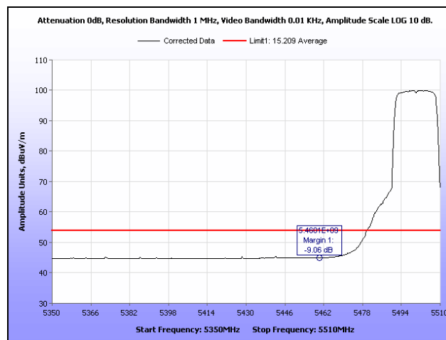
Plot 119. Restricted Band, 802.11a, 5500 MHz, Average
