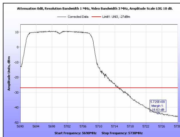
Plot 108. EIRP, 5700 MHz, 802.11a, Band Edge
