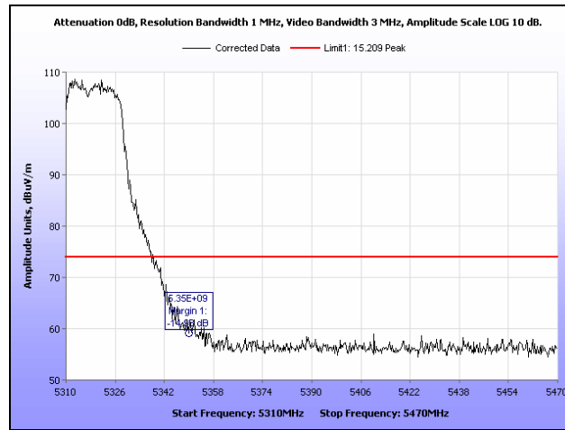
Plot 126. Restricted Band, 802.11n 40 MHz, 5310 MHz, Peak
