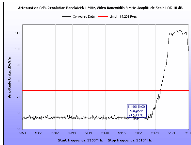
Plot 124. Restricted Band, 802.11n 20 MHz, 5500 MHz, Peak
