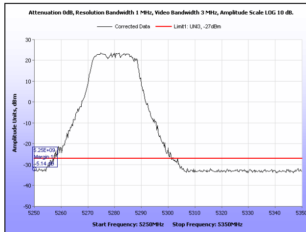
Plot 110. EIRP, 5280 MHz, 802.11n 20 MHz, Band Edge
