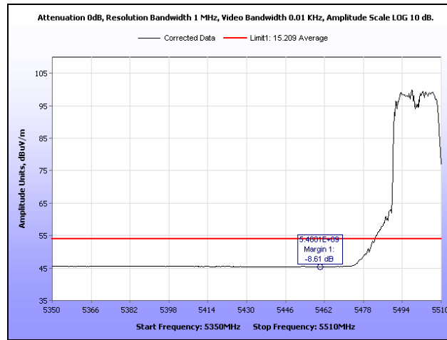
Plot 123. Restricted Band, 802.11n 20 MHz, 5500 MHz, Average
