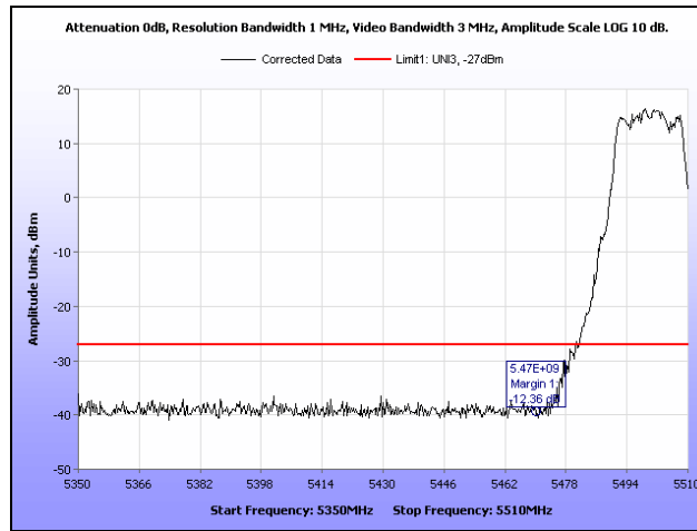
Plot 112. EIRP, 5500 MHz, 802.11n 20 MHz, Band Edge
