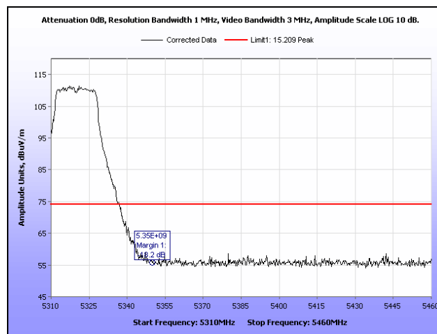
Plot 118. Restricted Band, 802.11a, 5320 MHz, Peak
