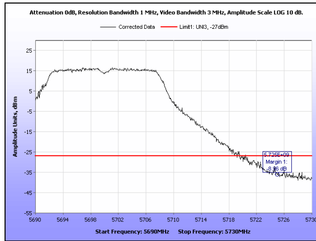
Plot 109. EIRP, 5700 MHz, 802.11a, Band Edge
