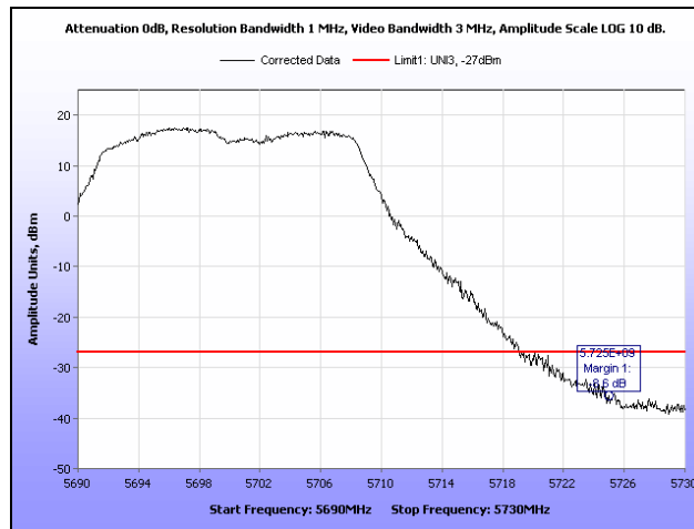
Plot 113. EIRP, 5700 MHz, 802.11n 20 MHz, Band Edge
