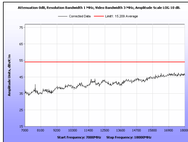
Plot 101. Radiated Spurious Emissions, 5795 MHz, 802.11n 40 MHz, 7 GHz – 18 GHz, Peak under Average
