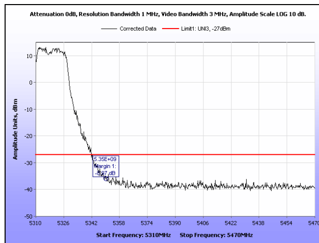
Plot 114. EIRP, 5310 MHz, 802.11n 40 MHz, Band Edge
