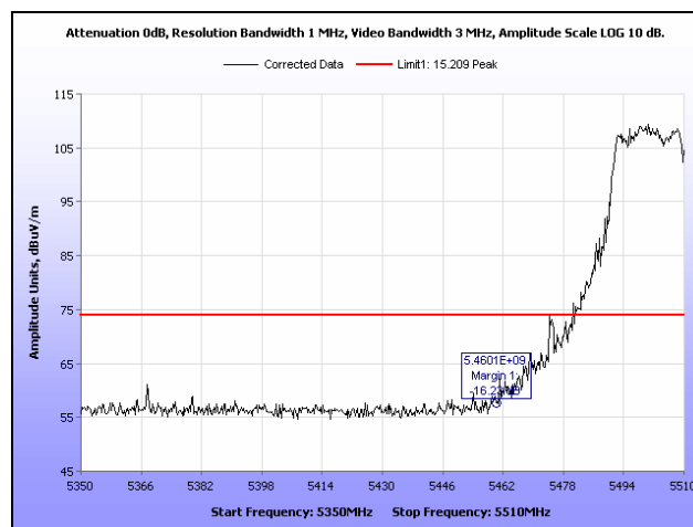
Plot 128. Restricted Band, 802.11n 40 MHz, 5510 MHz, Peak
