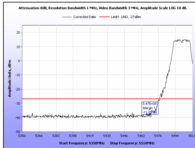
Plot 107. EIRP, 5500 MHz, 802.11a, Band Edge
