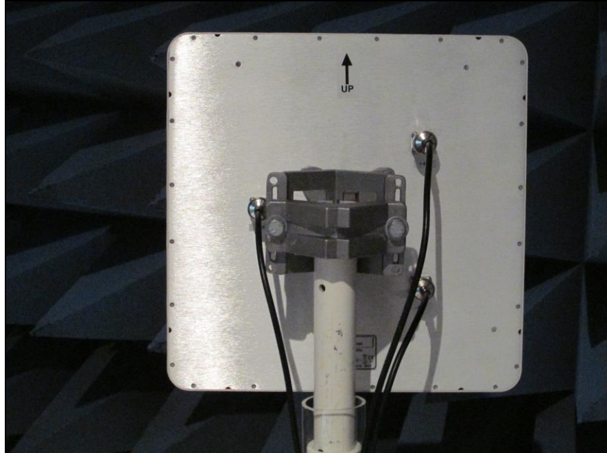
Photograph 3. Antenna Back
