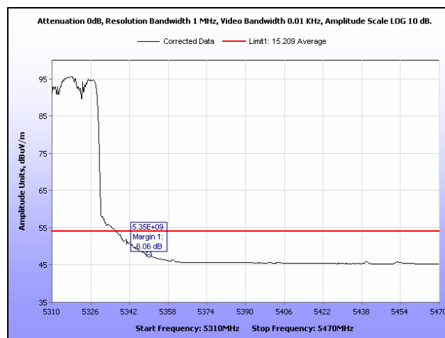
Plot 125. Restricted Band, 802.11n 40 MHz, 5310 MHz, Average
