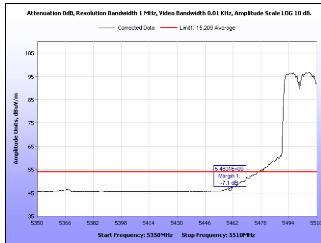
Plot 127. Restricted Band, 802.11n 40 MHz, 5510 MHz, Average
