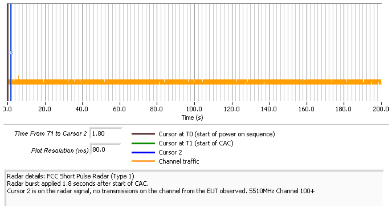
Figure 11 Radar Applied At Start of CAC (40MHz Bandwidth)
