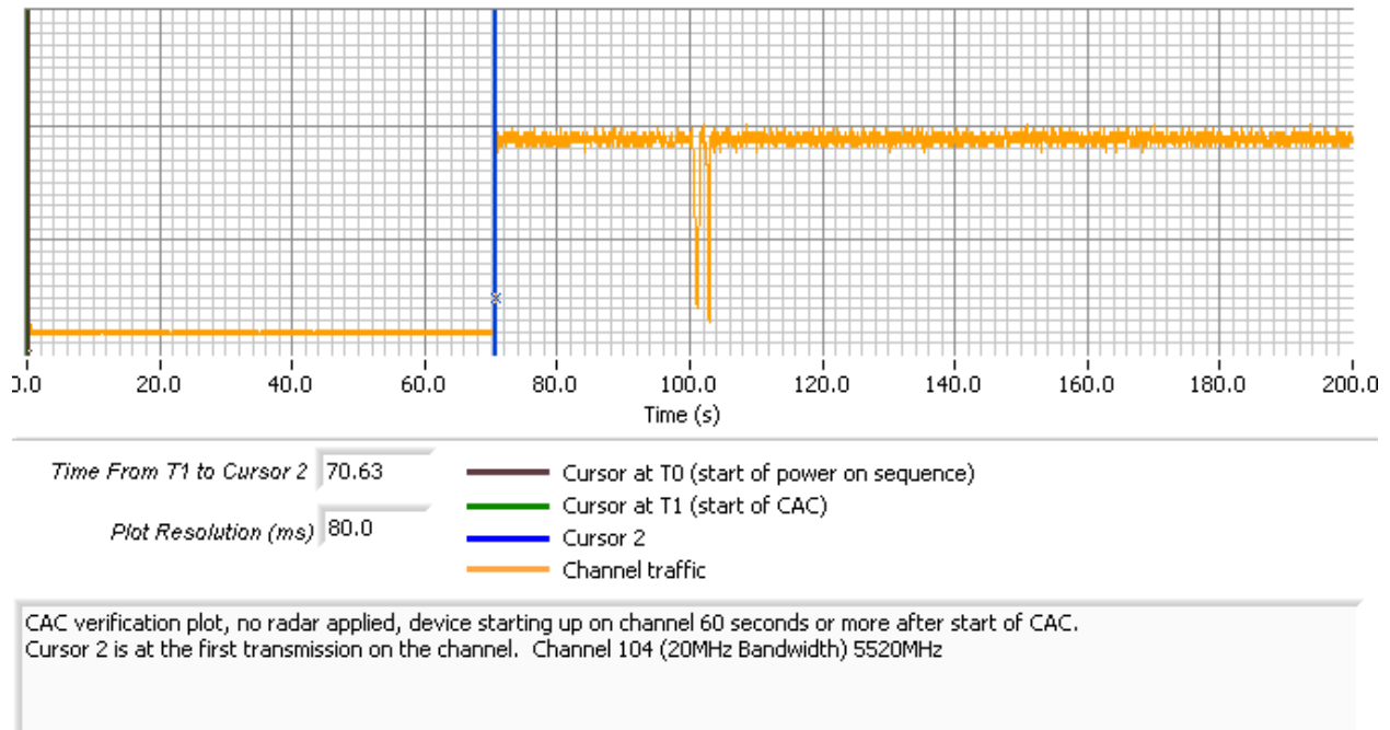
Figure 7 Plot of EUT Start-Up After CAC, 20MHz Bandwidth
