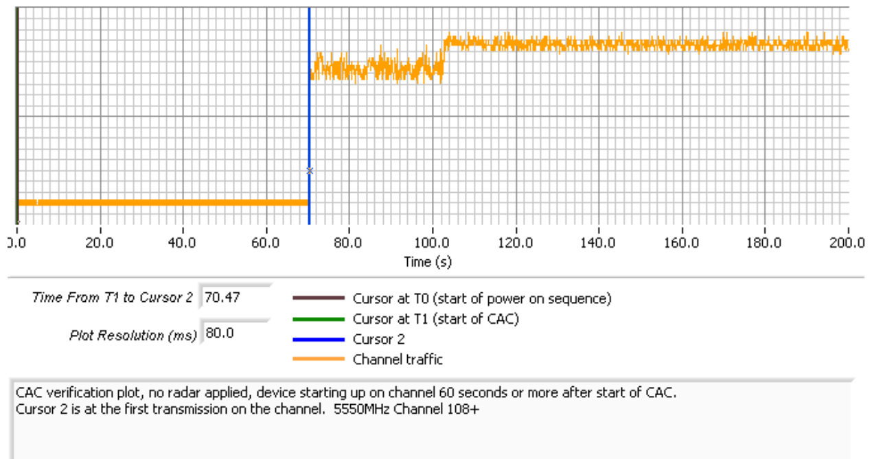
Figure 8 Plot of EUT Start-Up After CAC, 40MHz Bandwidth
