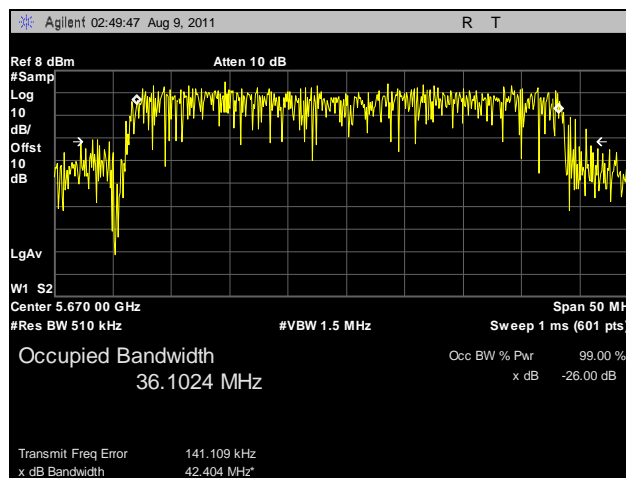
Plot 120. 99% Occupied Bandwidth, 802.11n HT40, 5670 MHz, R3-C
