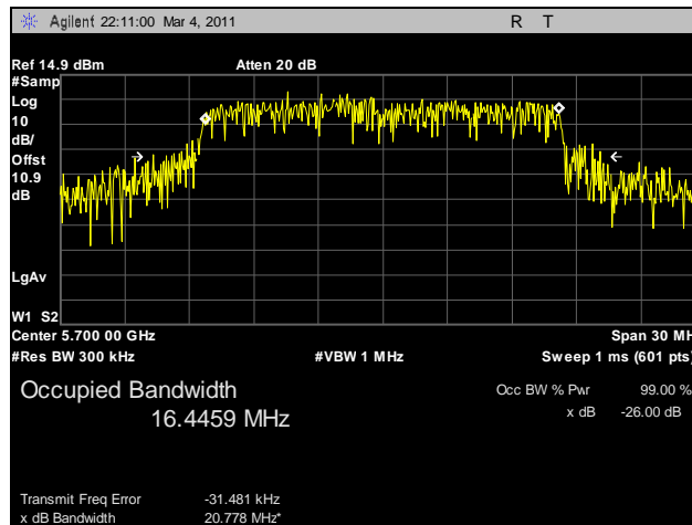
Plot 87. 99% Occupied Bandwidth, 802.11a, 5700 MHz, R3-C
