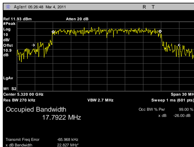
Plot 36. 26 dB Occupied Bandwidth, 802.11n HT20, 5320 MHz, R3-C
