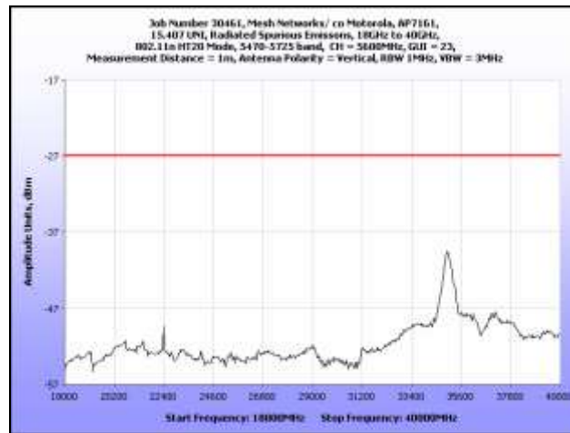
Plot 212. Radiated Spurious Emissions, 18 GHz – 40 GHz, 802.11n HT20, 5600 MHz
