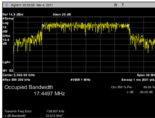
Plot 98. 99% Occupied Bandwidth, 802.11n HT20, 5500 MHz, R3-B
