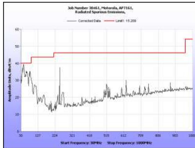
Plot 185. Radiated Spurious Emissions, 30 MHz – 1 GHz, 802.11a, 5580 MHz
