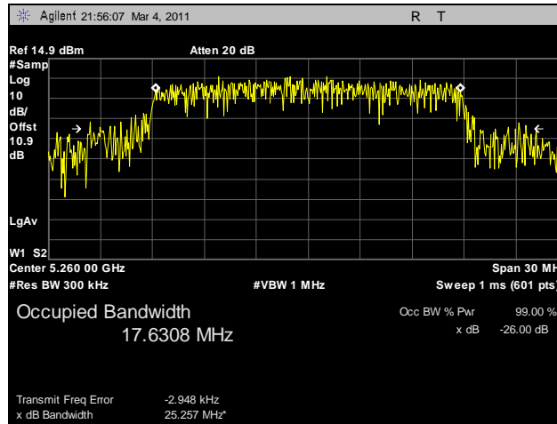
Plot 88. 99% Occupied Bandwidth, 802.11n HT20, 5260 MHz, R3-A
