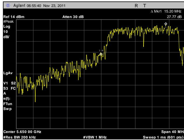
Plot 248. Radiated Band Edge, 802.11a, 5660 MHz, Port A
