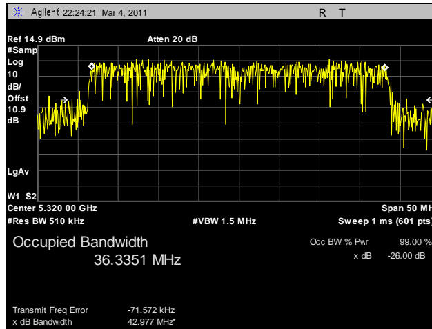
Plot 112. 99% Occupied Bandwidth, 802.11n HT40, 5320 MHz, R3-A
