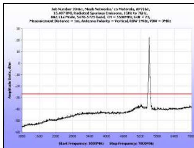
Plot 182. Radiated Spurious Emissions, 1 GHz – 7 GHz, 802.11a, 5500 MHz
