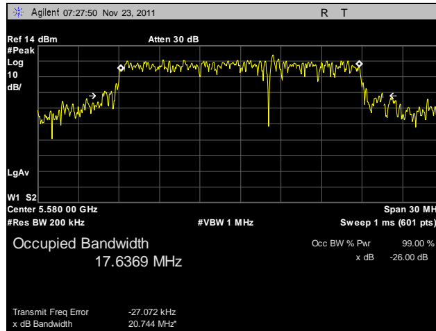
Plot 40. 26 dB Occupied Bandwidth, 802.11n HT20, 5580 MHz, R3-A
