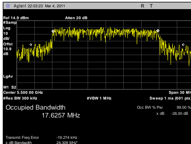
Plot 99. 99% Occupied Bandwidth, 802.11n HT20, 5500 MHz, R3-C
