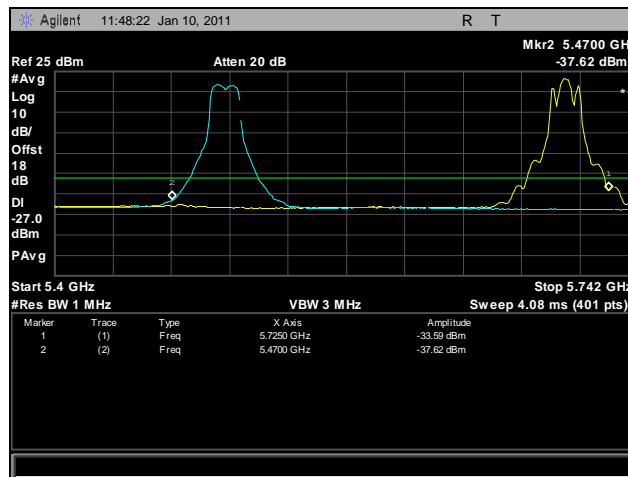
Plot 334. Frequency Stability, 20°C for 5470 MHz - 5725 MHz at 120 VAC
