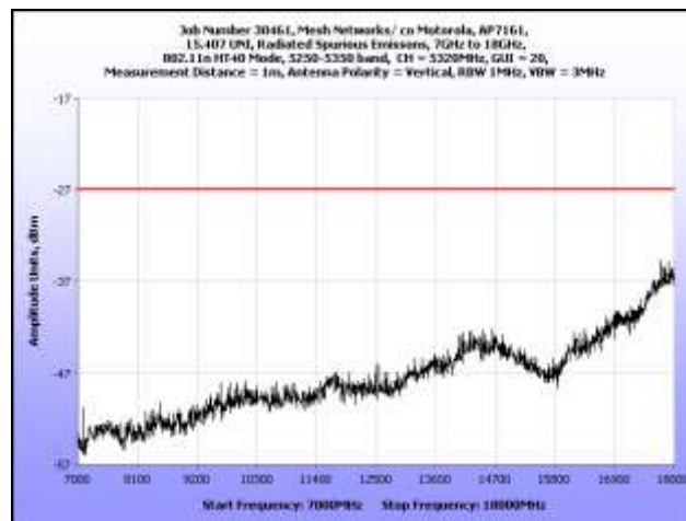
Plot 227. Radiated Spurious Emissions, 7 GHz – 18 GHz, 802.11n HT40, 5320 MHz
