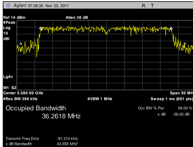
Plot 61. 26 dB Occupied Bandwidth, 802.11n HT40, 5580 MHz, R3-A
