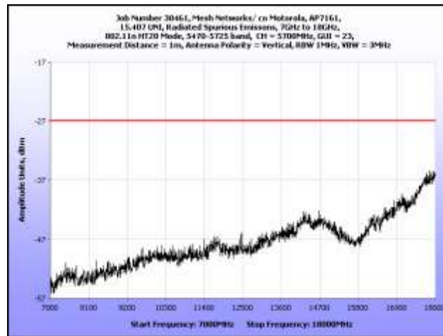
Plot 215. Radiated Spurious Emissions, 7 GHz – 18 GHz, 802.11n HT20, 5700 MHz
