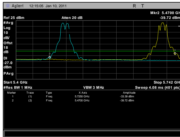
Plot 340. Frequency Stability, 40°C for 5470 MHz - 5725 MHz at 120 VAC
