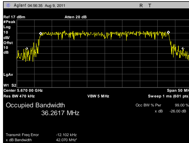
Plot 64. 26 dB Occupied Bandwidth, 802.11n HT40, 5670 MHz, R3-A
