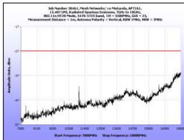
Plot 207. Radiated Spurious Emissions, 7 GHz – 18 GHz, 802.11n HT20, 5500 MHz
