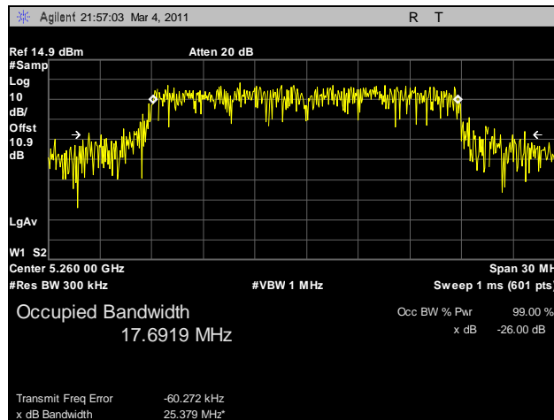
Plot 90. 99% Occupied Bandwidth, 802.11n HT20, 5260 MHz, R3-C
