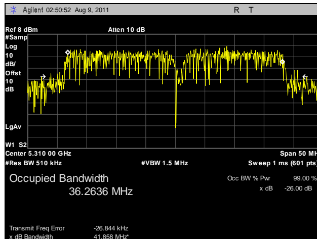
Plot 111. 99% Occupied Bandwidth, 802.11n HT40, 5310 MHz, R3-C
