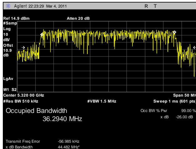
Plot 114. 99% Occupied Bandwidth, 802.11n HT40, 5320 MHz, R3-C
