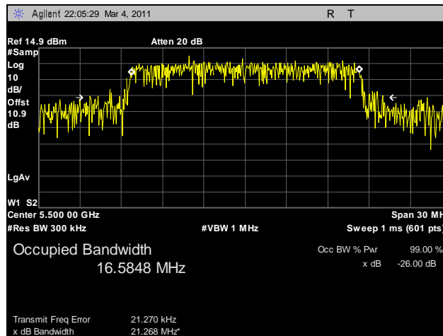
Plot 81. 99% Occupied Bandwidth, 802.11a, 5500 MHz, R3-C
