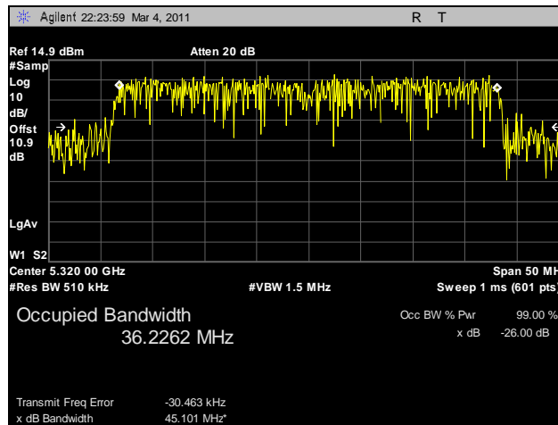
Plot 113. 99% Occupied Bandwidth, 802.11n HT40, 5320 MHz, R3-B
