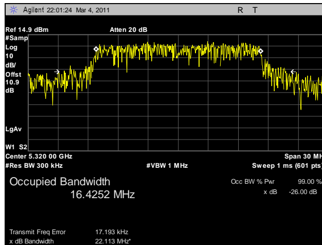
Plot 77. 99% Occupied Bandwidth, 802.11a, 5320 MHz, R3-B
