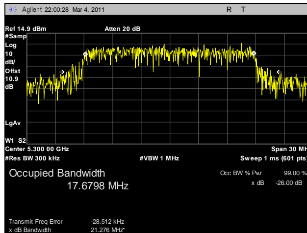
Plot 93. 99% Occupied Bandwidth, 802.11n HT20, 5300 MHz, R3-C
