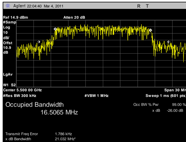
Plot 79. 99% Occupied Bandwidth, 802.11a, 5500 MHz, R3-A
