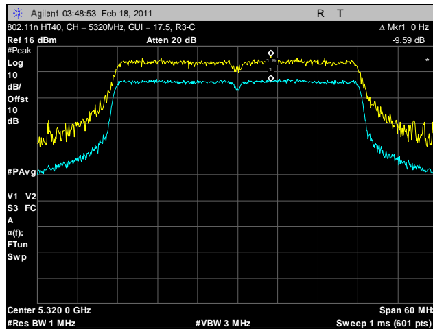
Plot 162. Peak Excursion Ratio, 802.11n HT40, 5320 MHz, R3-C
