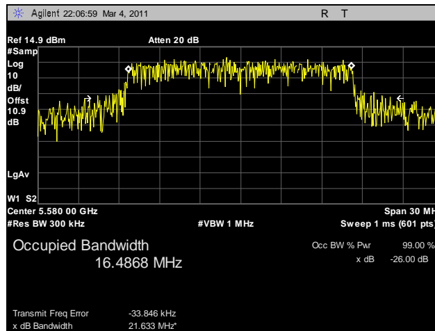
Plot 83. 99% Occupied Bandwidth, 802.11a, 5580 MHz, R3-B
