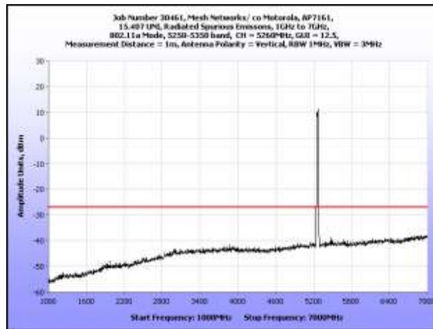
Plot 170. Radiated Spurious Emissions, 1 GHz – 7 GHz, 802.11a, 5260 MHz
