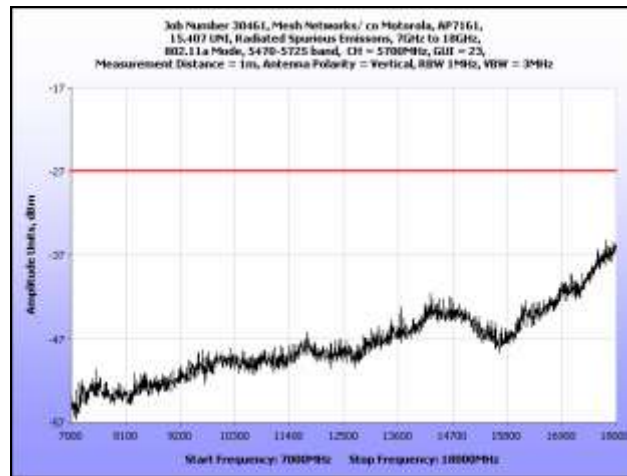
Plot 191. Radiated Spurious Emissions, 7 GHz – 18 GHz, 802.11a, 5700 MHz
