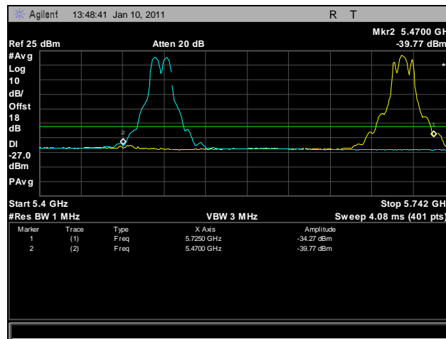
Plot 319. Frequency Stability, -30°C for 5470 MHz - 5725 MHz at 120 VAC
