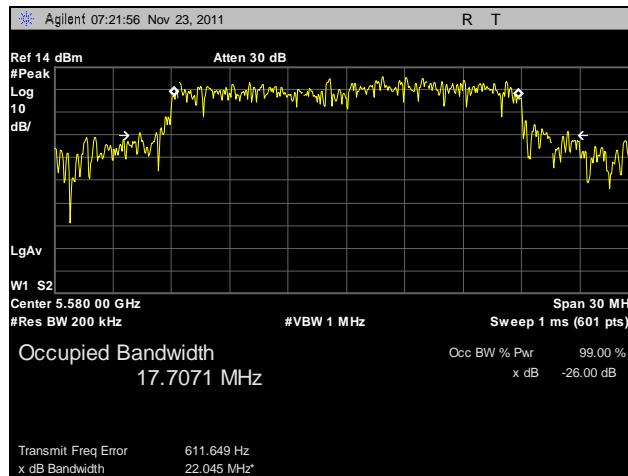
Plot 41. 26 dB Occupied Bandwidth, 802.11n HT20, 5580 MHz, R3-B
