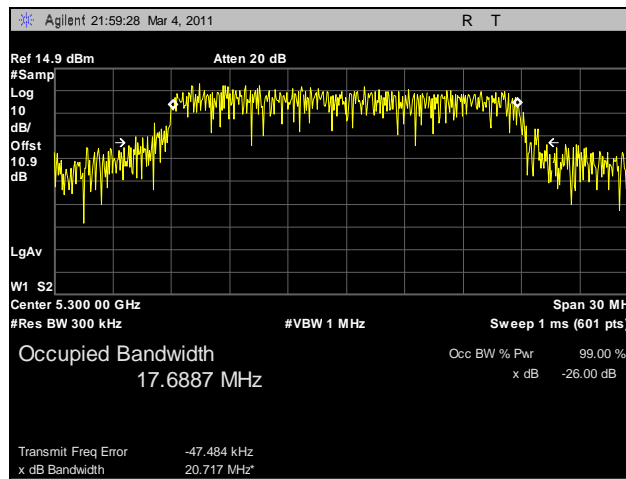
Plot 92. 99% Occupied Bandwidth, 802.11n HT20, 5300 MHz, R3-B
