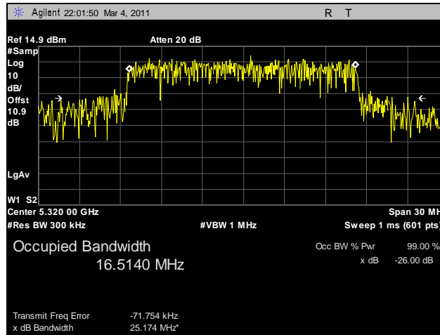
Plot 76. 99% Occupied Bandwidth, 802.11a, 5320 MHz, R3-A
