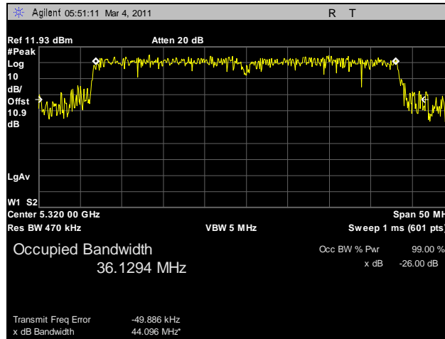
Plot 55. 26 dB Occupied Bandwidth, 802.11n HT40, 5320 MHz, R3-A
