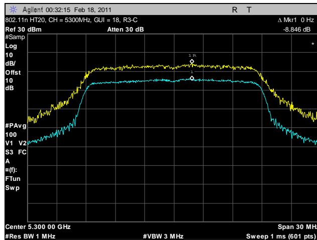
Plot 144. Peak Excursion Ratio, 802.11n HT20, 5300 MHz, R3-C
