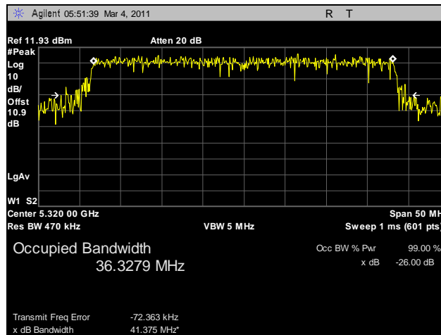
Plot 56. 26 dB Occupied Bandwidth, 802.11n HT40, 5320 MHz, R3-B
