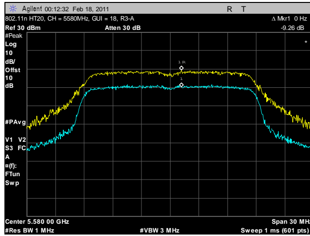
Plot 151. Peak Excursion Ratio, 802.11n HT20, 5580 MHz, R3-A
