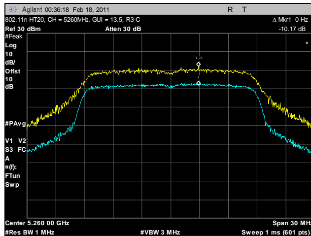
Plot 141. Peak Excursion Ratio, 802.11n HT20, 5260 MHz, R3-C
