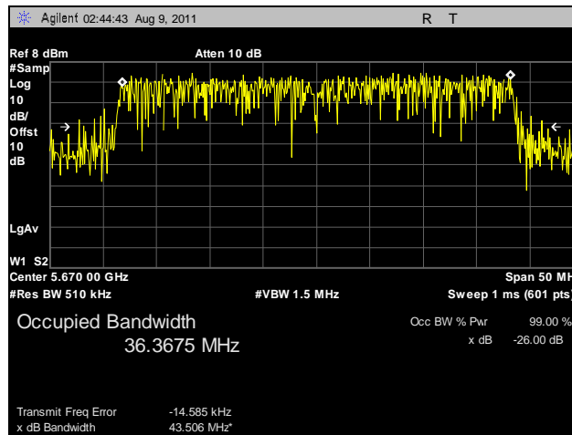
Plot 118. 99% Occupied Bandwidth, 802.11n HT40, 5670 MHz, R3-A
