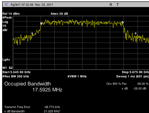
Plot 44. 26 dB Occupied Bandwidth, 802.11n HT20, 5660 MHz, R3-B
