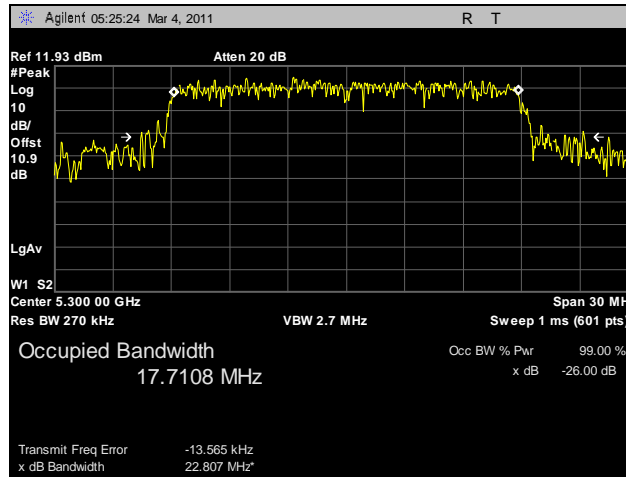
Plot 31. 26 dB Occupied Bandwidth, 802.11n HT20, 5300 MHz, R3-A
