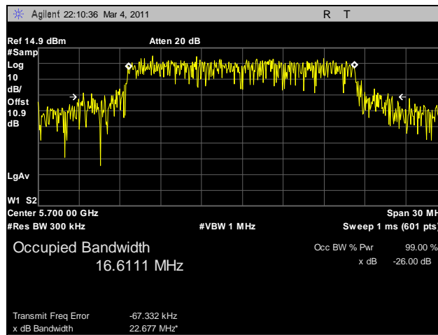
Plot 86. 99% Occupied Bandwidth, 802.11a, 5700 MHz, R3-B
