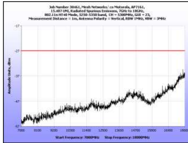
Plot 223. Radiated Spurious Emissions, 7 GHz – 18 GHz, 802.11n HT40, 5300 MHz
