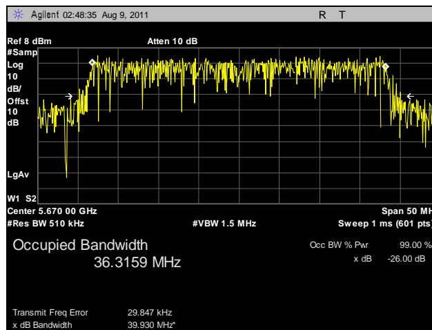
Plot 119. 99% Occupied Bandwidth, 802.11n HT40, 5670 MHz, R3-B
