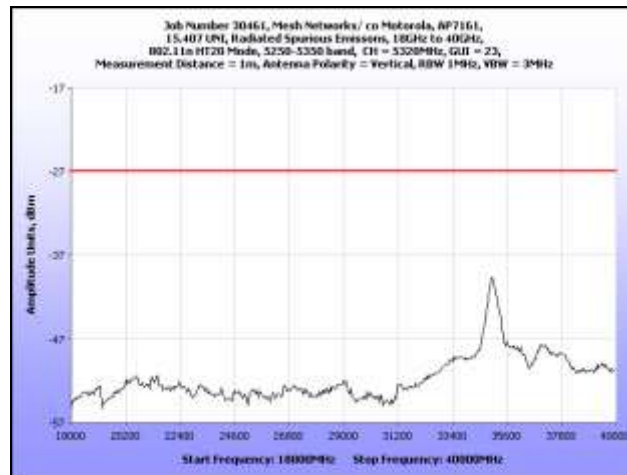
Plot 204. Radiated Spurious Emissions, 18 GHz – 40 GHz, 802.11n HT20, 5320 MHz
