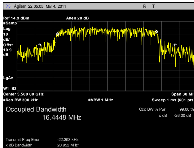
Plot 80. 99% Occupied Bandwidth, 802.11a, 5500 MHz, R3-B
