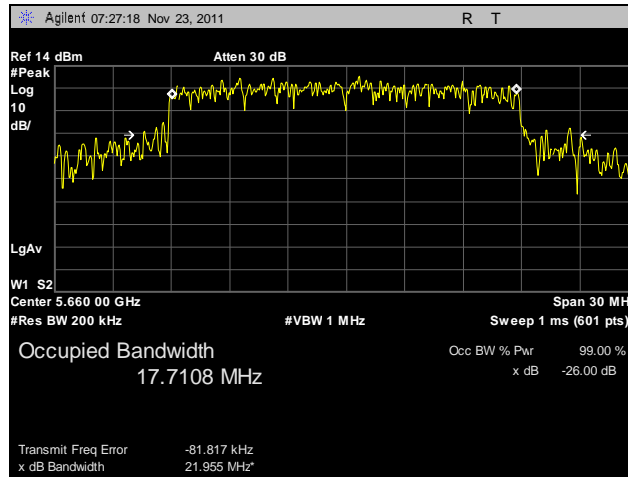
Plot 43. 26 dB Occupied Bandwidth, 802.11n HT20, 5660 MHz, R3-A
