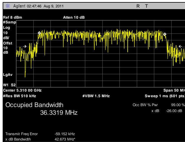
Plot 110. 99% Occupied Bandwidth, 802.11n HT40, 5310 MHz, R3-B
