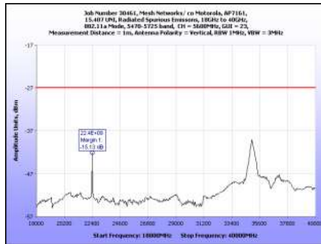
Plot 188. Radiated Spurious Emissions, 18 GHz – 40 GHz, 802.11a, 5600 MHz
