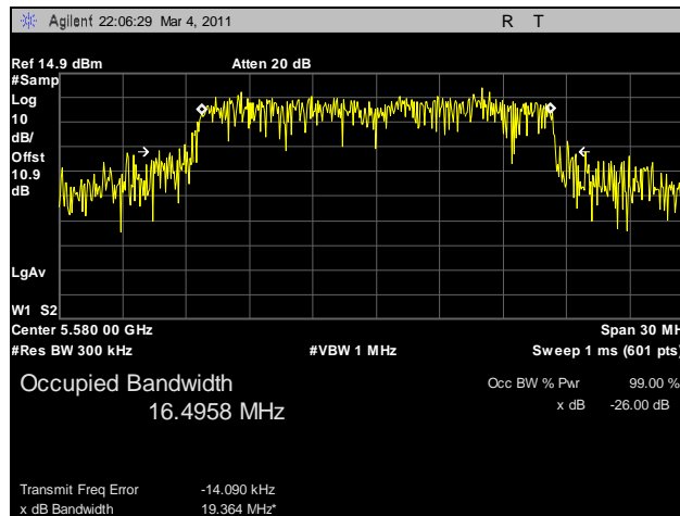
Plot 84. 99% Occupied Bandwidth, 802.11a, 5580 MHz, R3-C
