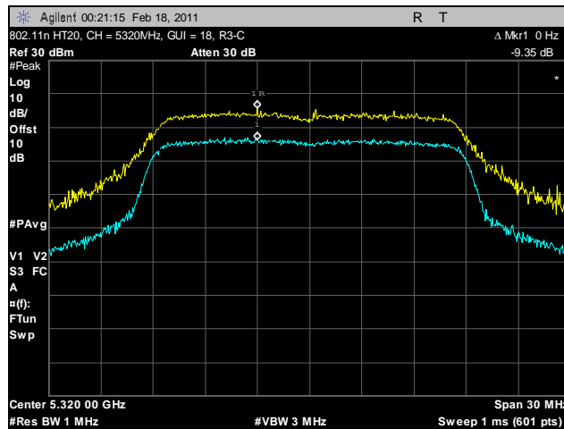
Plot 147. Peak Excursion Ratio, 802.11n HT20, 5320 MHz, R3-C
