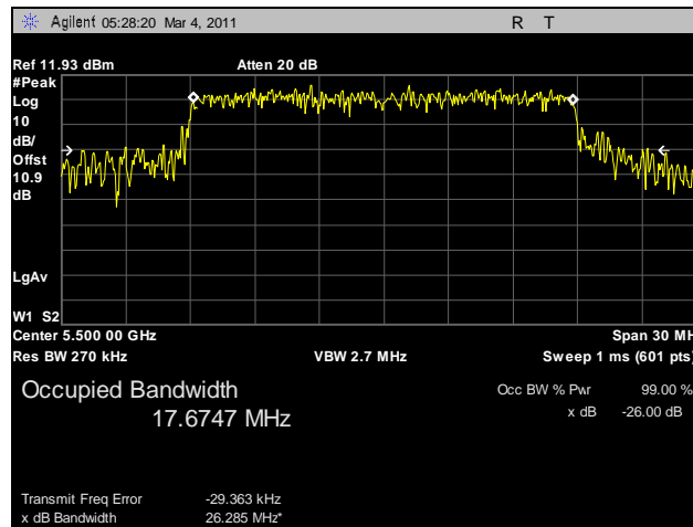
Plot 37. 26 dB Occupied Bandwidth, 802.11n HT20, 5500 MHz, R3-A
