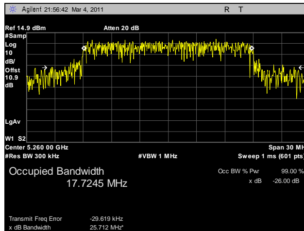
Plot 89. 99% Occupied Bandwidth, 802.11n HT20, 5260 MHz, R3-B
