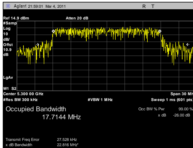
Plot 91. 99% Occupied Bandwidth, 802.11n HT20, 5300 MHz, R3-A
