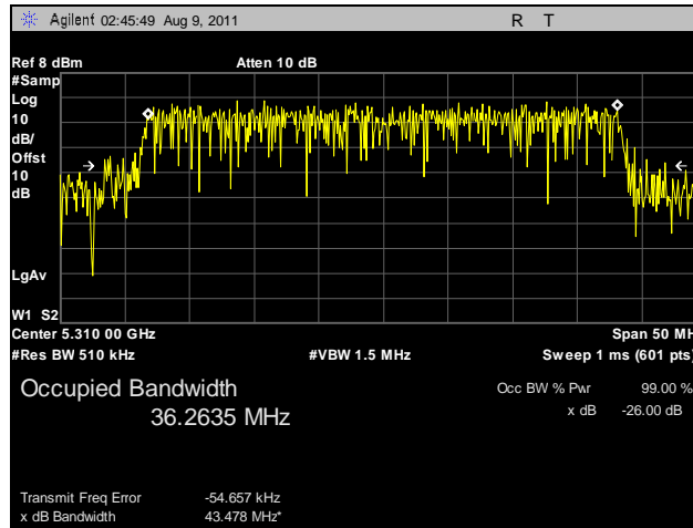
Plot 109. 99% Occupied Bandwidth, 802.11n HT40, 5310 MHz, R3-A
