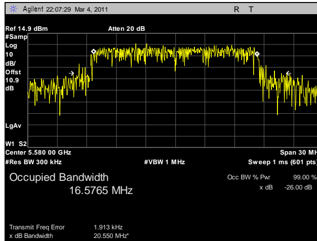
Plot 82. 99% Occupied Bandwidth, 802.11a, 5580 MHz, R3-A
