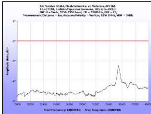
Plot 176. Radiated Spurious Emissions, 18 GHz – 40 GHz, 802.11a, 5300 MHz
