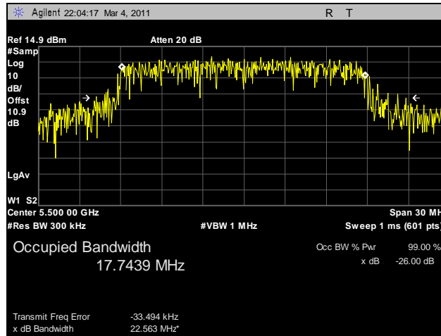
Plot 97. 99% Occupied Bandwidth, 802.11n HT20, 5500 MHz, R3-A
