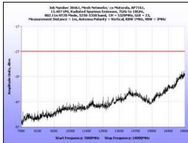
Plot 203. Radiated Spurious Emissions, 7 GHz – 18 GHz, 802.11n HT20, 5320 MHz
