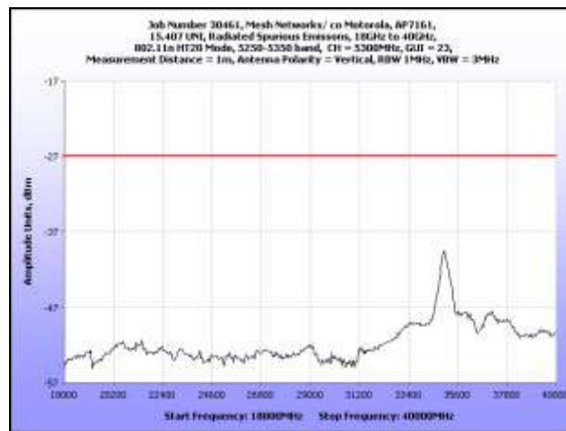
Plot 200. Radiated Spurious Emissions, 18 GHz – 40 GHz, 802.11n HT20, 5300 MHz
