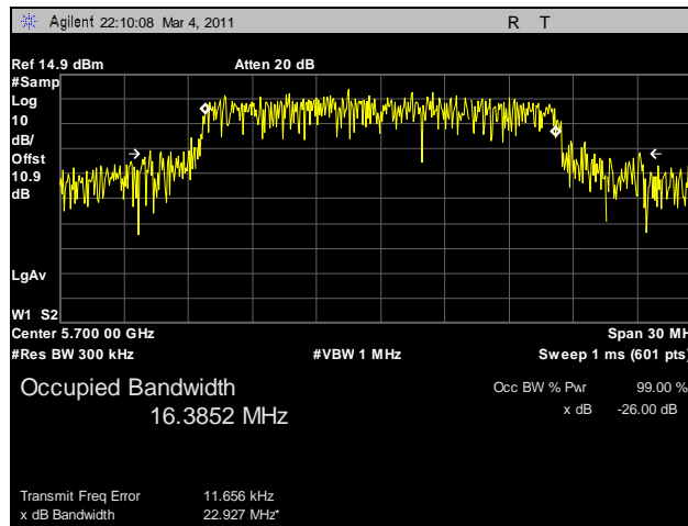
Plot 85. 99% Occupied Bandwidth, 802.11a, 5700 MHz, R3-A
