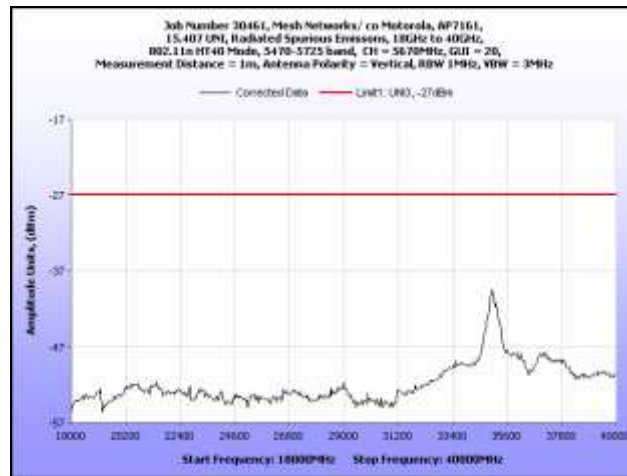
Plot 236. Radiated Spurious Emissions, 18 GHz – 40 GHz, 802.11n HT40, 5670 MHz
