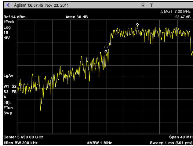
Plot 262. Radiated Band Edge, 802.11n HT20, 5660 MHz, Port A
