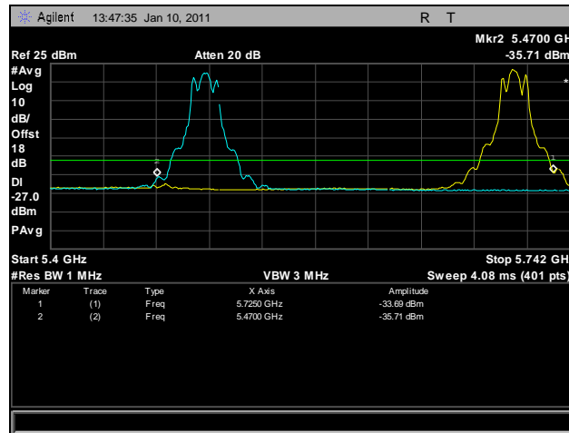
Plot 318. Frequency Stability, -30°C for 5470 MHz - 5725 MHz at 102 VAC
