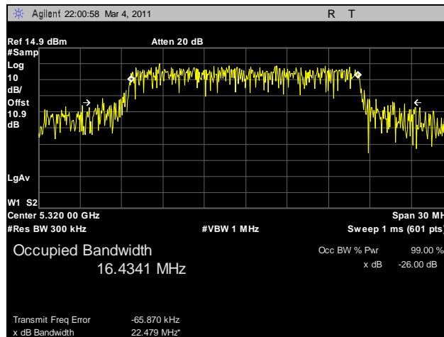
Plot 78. 99% Occupied Bandwidth, 802.11a, 5320 MHz, R3-C
