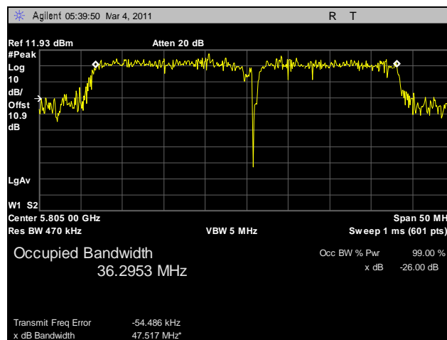
Plot 33. 26 dB Occupied Bandwidth, 802.11n 40 MHz, High Channel, Port C
