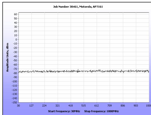
Plot 183. Receiver Spurious Emission 5.8 GHz, Port C, 30 MHz – 1 GHz
