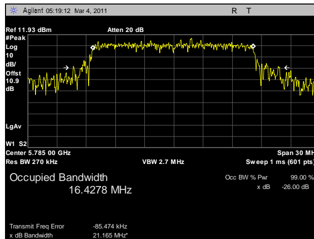
Plot 11. 26 dB Occupied Bandwidth, 802.11a, Mid Channel, Port B
