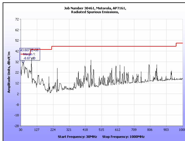
Plot 96. Radiated Spurious Emissions, 802.11a, High Channel, 30 MHz – 1 GHz
