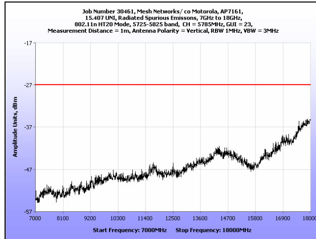
Plot 106. Radiated Spurious Emissions, 802.11n 20 MHz, Mid Channel, 7 GHz – 18 GHz
