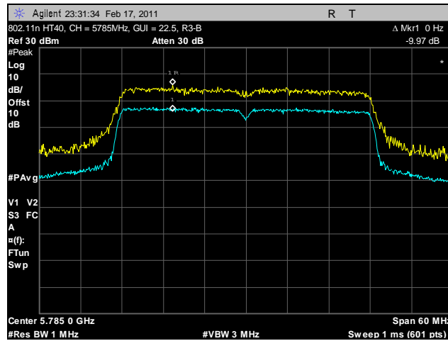
Plot 83. Peak Excursion Ratio, 802.11n 40 MHz, Mid Channel, Port B
