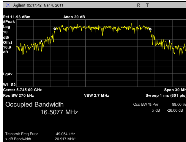
Plot 13. 26 dB Occupied Bandwidth, 802.11a, Low Channel, Port C
