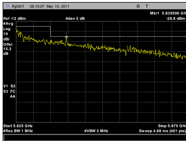
Plot 137. Band Edge, 802.11n HT40, High Channel, Port A
