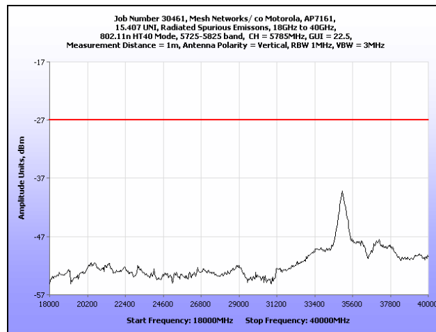
Plot 119. Radiated Spurious Emissions, 802.11n 40 MHz, Mid Channel, 18 GHz – 40 GHz
