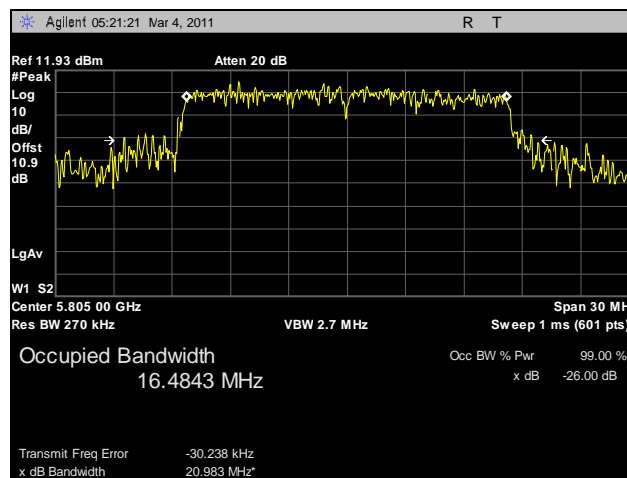
Plot 12. 26 dB Occupied Bandwidth, 802.11a, High Channel, Port B
