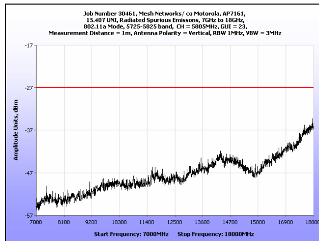
Plot 98. Radiated Spurious Emissions, 802.11a, High Channel, 7 GHz – 18 GHz
