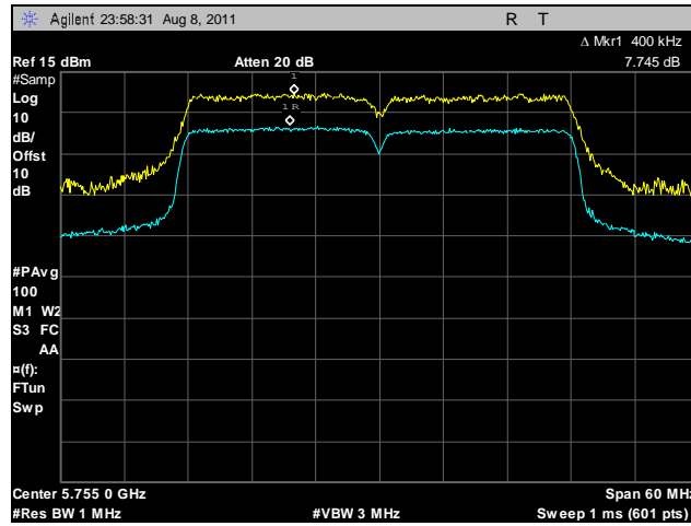
Plot 82. Peak Excursion Ratio, 802.11n 40 MHz, Low Channel, Port B
