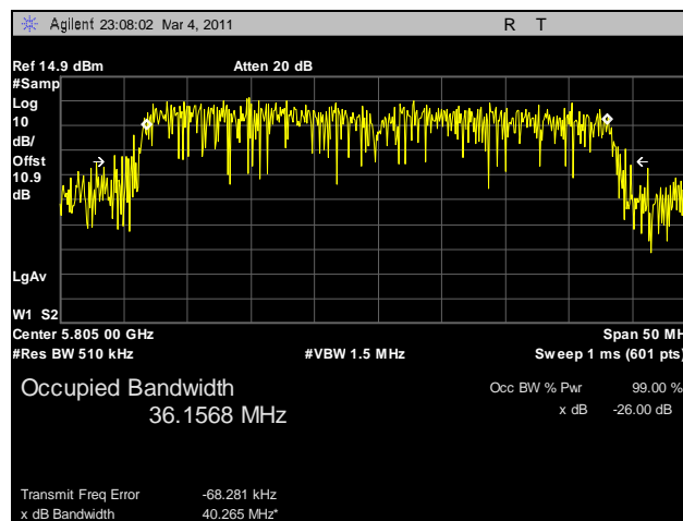
Plot 57. 99% Occupied Bandwidth, 802.11n 40 MHz, High Channel, Port B
