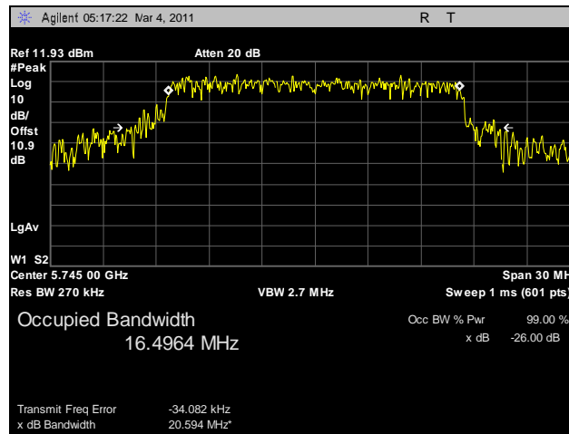
Plot 10. 26 dB Occupied Bandwidth, 802.11a, Low Channel, Port B
