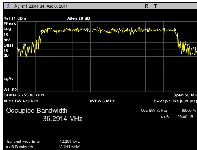
Plot 31. 26 dB Occupied Bandwidth, 802.11n 40 MHz, Low Channel, Port C
