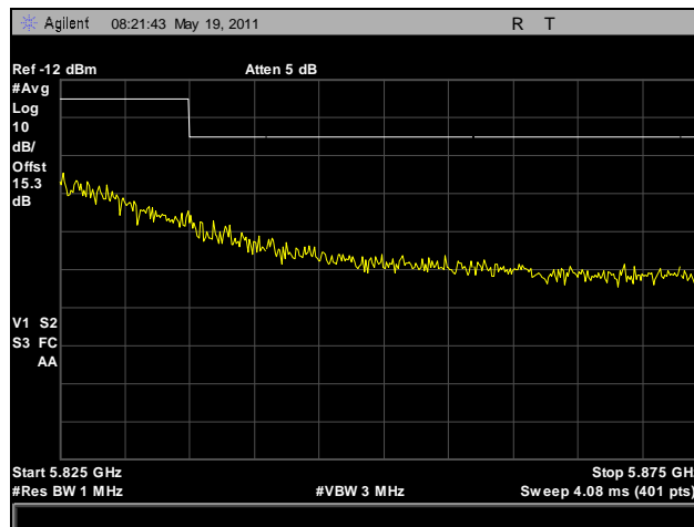
Plot 125. Band Edge, 802.11a, High Channel, Port A
