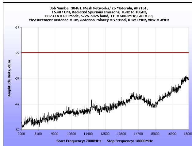
Plot 110. Radiated Spurious Emissions, 802.11n 20 MHz, High Channel, 7 GHz – 18 GHz
