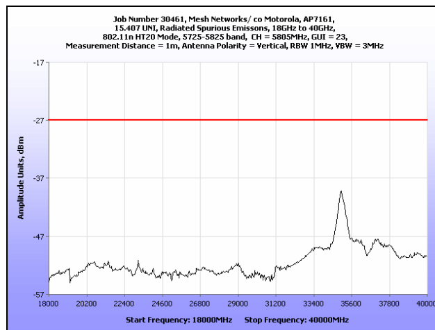
Plot 111. Radiated Spurious Emissions, 802.11n 20 MHz, High Channel, 18 GHz – 40 GHz
