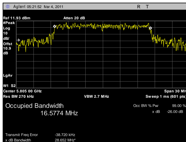
Plot 15. 26 dB Occupied Bandwidth, 802.11a, High Channel, Port C
