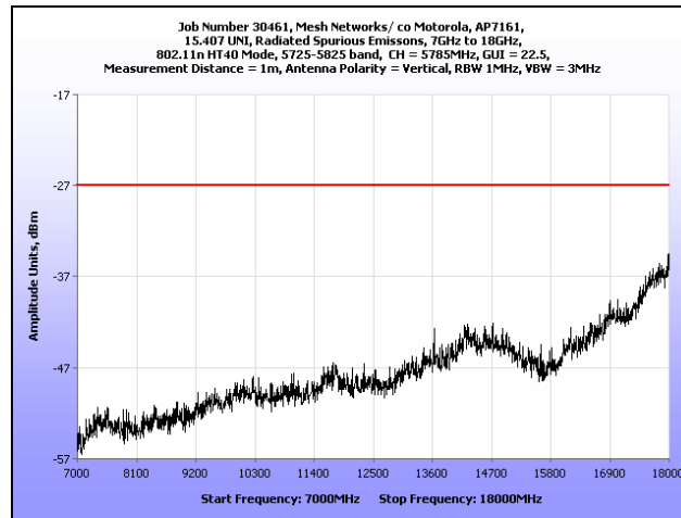
Plot 118. Radiated Spurious Emissions, 802.11n 40 MHz, Mid Channel, 7 GHz – 18 GHz
