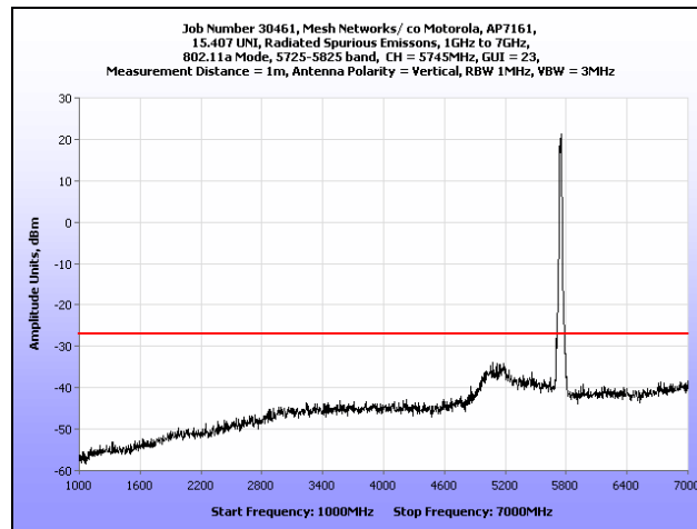
Plot 89. Radiated Spurious Emissions, 802.11a, Low Channel, 1 GHz – 7 GHz
