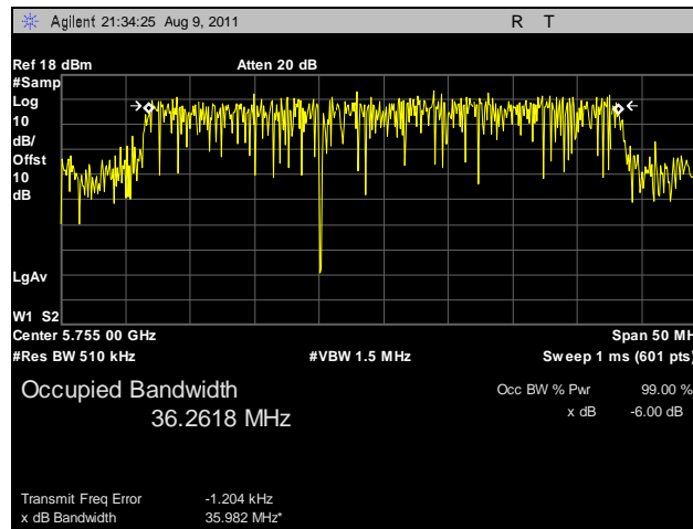
Plot 55. 99% Occupied Bandwidth, 802.11n 40 MHz, Low Channel, Port B
