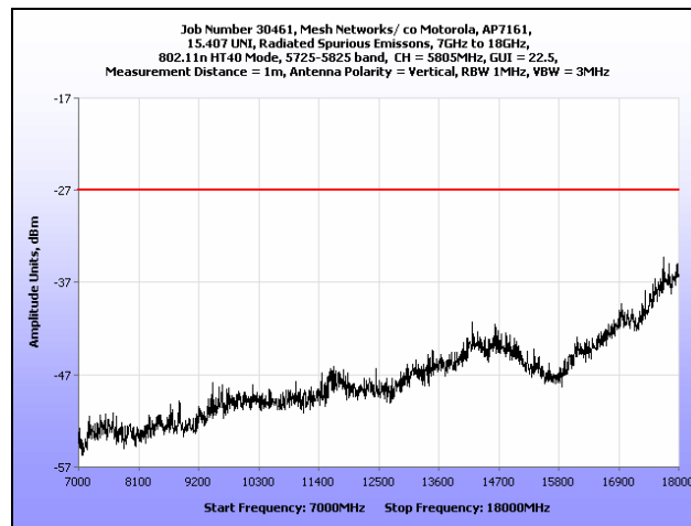
Plot 122. Radiated Spurious Emissions, 802.11n 40 MHz, High Channel, 7 GHz – 18 GHz
