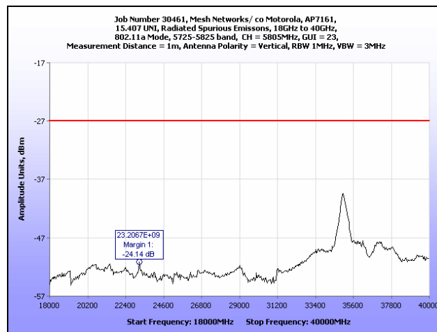
Plot 99. Radiated Spurious Emissions, 802.11a, High Channel, 18 GHz – 40 GHz
