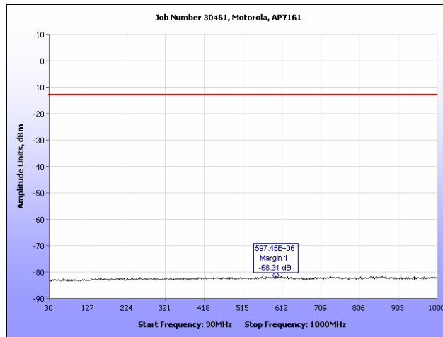
Plot 77. Conducted Spurious Emissions, 802.11a, 4960 MHz (30 MHz - 1 GHz), R3-B
