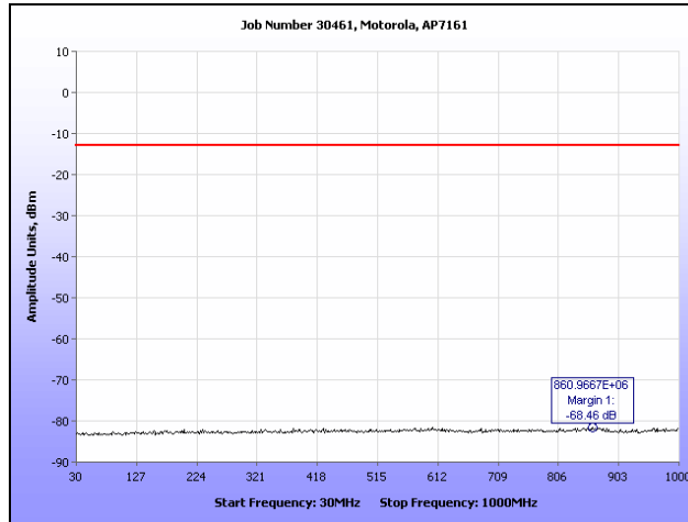
Plot 95. Conducted Spurious Emissions, 802.11a, 4980 MHz (30 MHz – 1 GHz), R3-B
