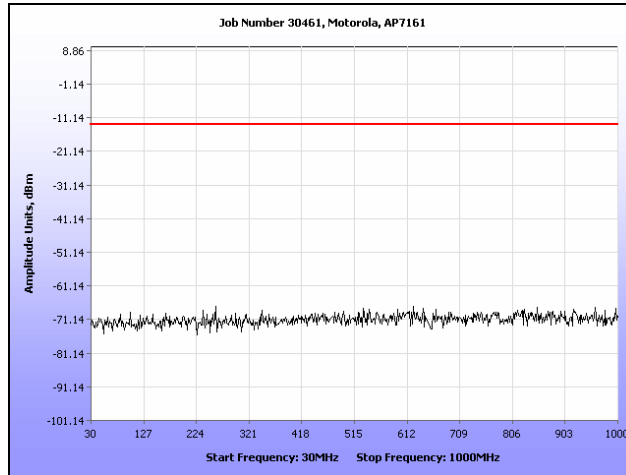
Plot 146. Conducted Spurious Emissions, 802.11a, 4980 MHz (30 MHz – 1 GHz), (1x1)
