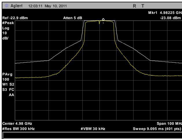
Plot 43. Emission Mask, 802.11a, 4980 MHz, Port B (3x3)
