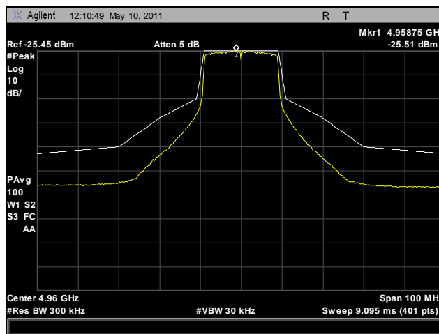
Plot 50. Emission Mask, 802.11n HT20, 4960 MHz, Port C (3x3)
