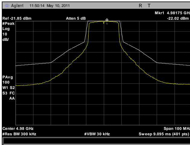
Plot 42. Emission Mask, 802.11a, 4980 MHz, Port A (3x3)
