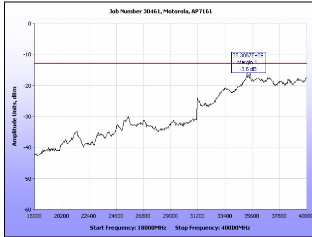
Plot 194. Radiated Spurious Emissions, 802.11n HT20, 4950 MHz (18 GHz – 40 GHz), (1x1)
