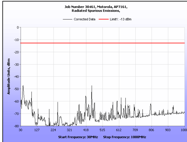
Plot 167. Radiated Spurious Emissions, 802.11a, 4970 MHz (30 MHz – 1 GHz)
