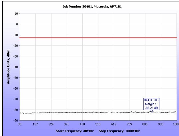
Plot 110. Conducted Spurious Emissions, 802.11n HT20, 4960 MHz (30 MHz – 1 GHz), R3-A
