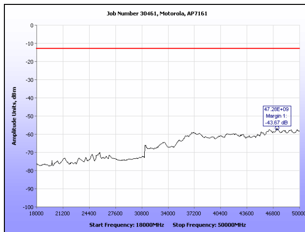
Plot 121. Conducted Spurious Emissions, 802.11n HT20, 4970 MHz (18 GHz – 50 GHz), R3-A
