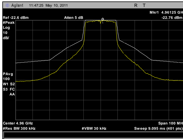
Plot 48. Emission Mask, 802.11n HT20, 4960 MHz, Port A (3x3)
