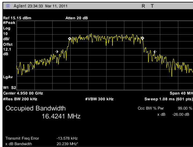
Plot 1. Emission Bandwidth, 802.11a, 4950 MHz, Port A (3x3)
