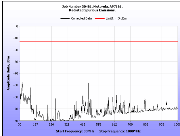
Plot 176. Radiated Spurious Emissions, 802.11n HT20, 4960 MHz (30 MHz – 1 GHz)
