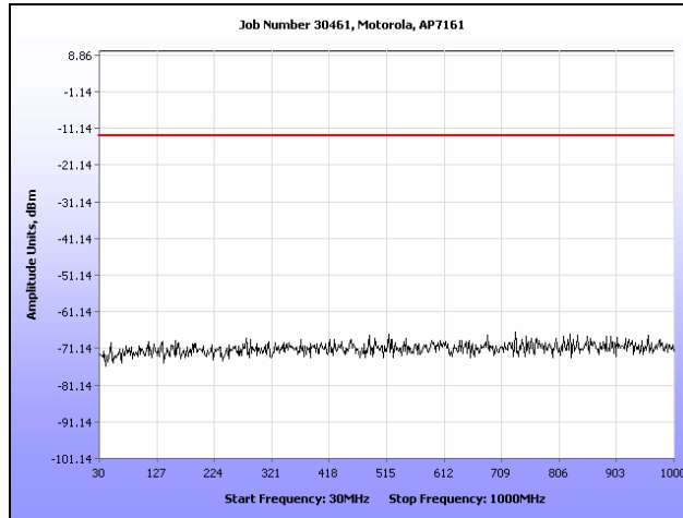
Plot 149. Conducted Spurious Emissions, 802.11n HT20, 4950 MHz (30 MHz – 1 GHz), (1x1)
