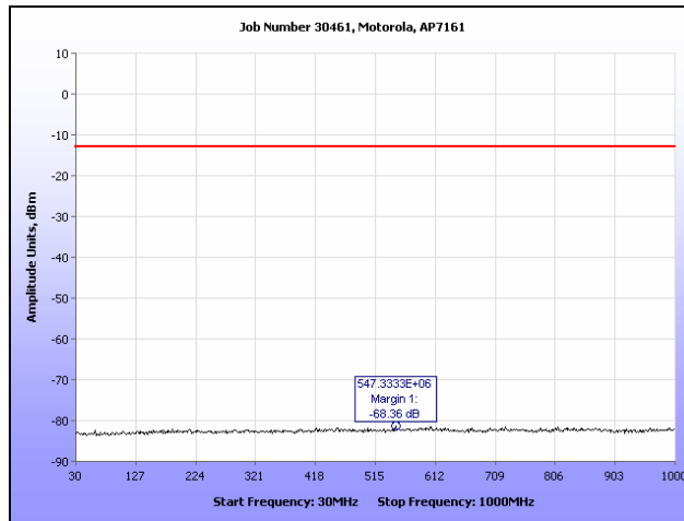
Plot 122. Conducted Spurious Emissions, 802.11n HT20, 4970 MHz (30 MHz - 1 GHz), R3-B
