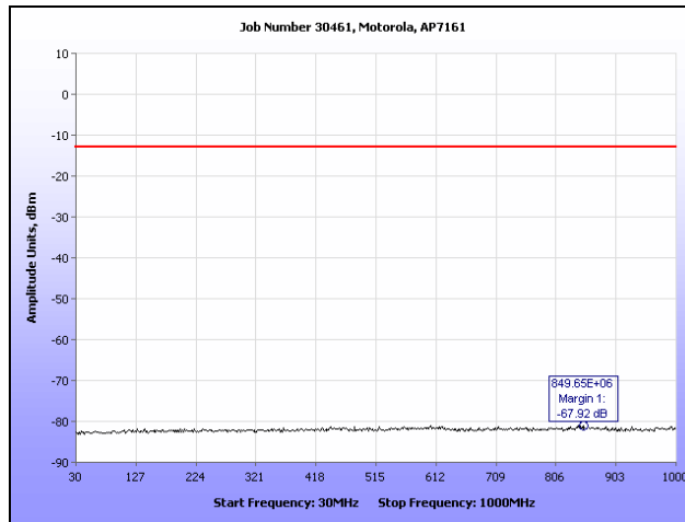
Plot 83. Conducted Spurious Emissions, 802.11a, 4970 MHz (30 MHz – 1 GHz), R3-A
