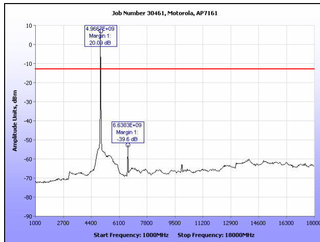
Plot 90. Conducted Spurious Emissions, 802.11a, 4970 MHz (1 GHz – 18 GHz), R3-C
