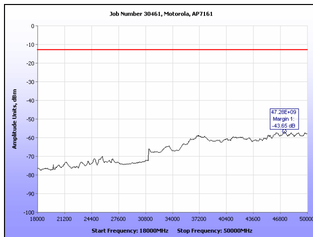
Plot 91. Conducted Spurious Emissions, 802.11a, 4970 MHz (18 GHz – 50 GHz), R3-C
