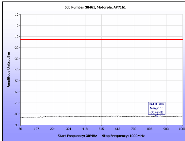
Plot 80. Conducted Spurious Emissions, 802.11a, 4960 MHz (30 MHz – 1 GHz), R3-C
