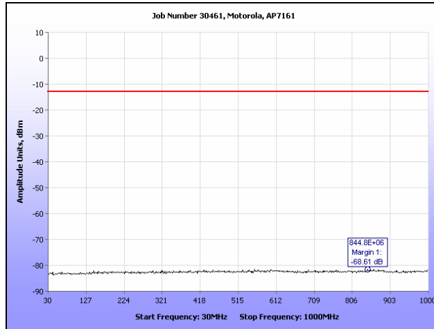
Plot 113. Conducted Spurious Emissions, 802.11n HT20, 4960 MHz (30 MHz - 1 GHz), R3-B
