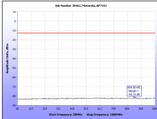
Plot 92. Conducted Spurious Emissions, 802.11a, 4980 MHz (30 MHz – 1 GHz), R3-A
