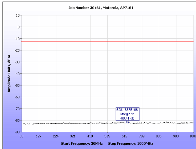
Plot 89. Conducted Spurious Emissions, 802.11a, 4970 MHz (30 MHz – 1 GHz), R3-C
