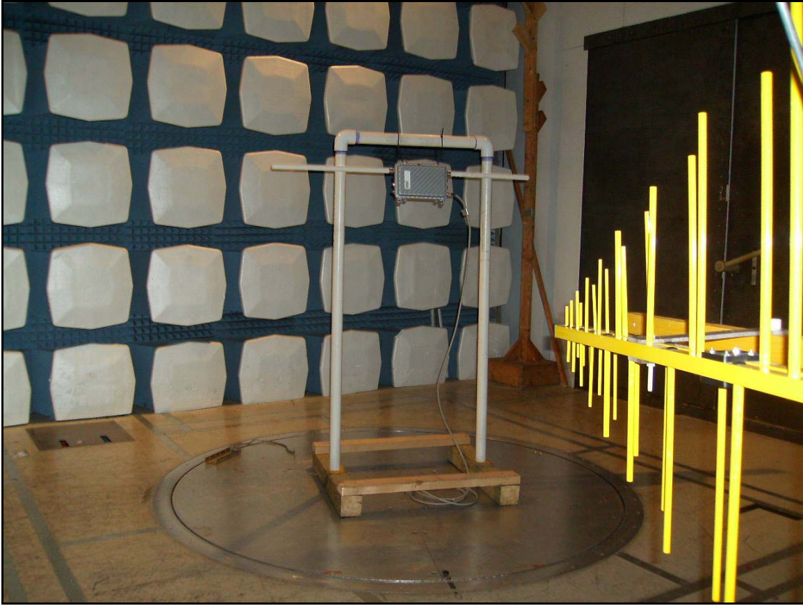
Photograph 2. Test Setup Photo, Radiated Emissions
